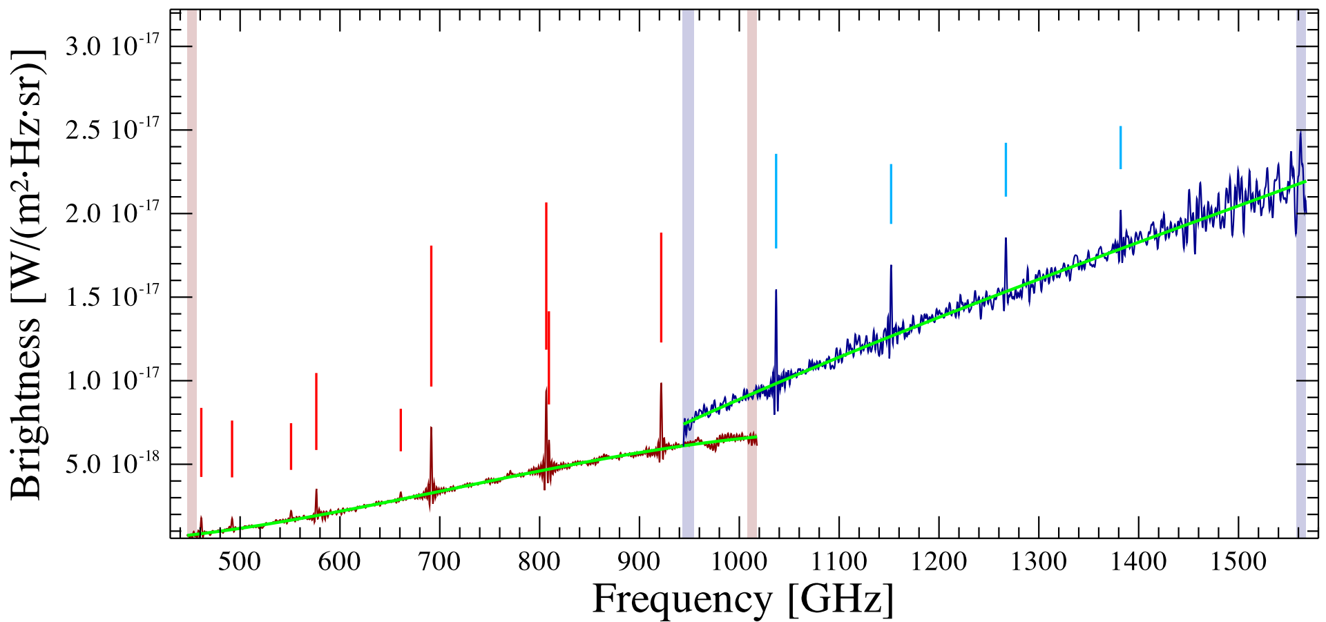
Ced110 IRS 4 Observation ID 1342248246; (9/4)
