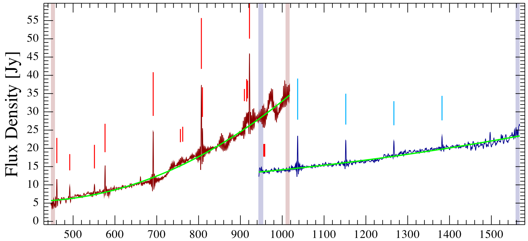
Ced110 IRS 4 Observation ID 1342248246; (9/4)
