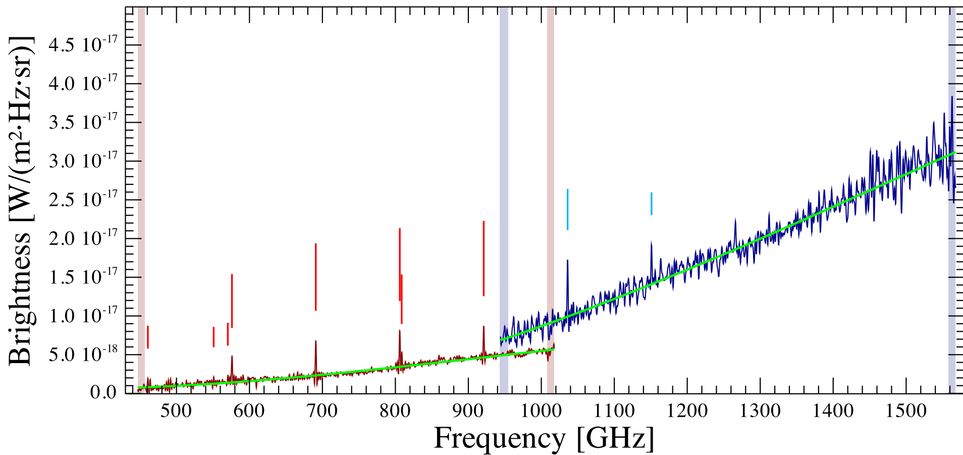
SAGE045400.9-691151.6 Observation ID 1342248242; (8/2)
