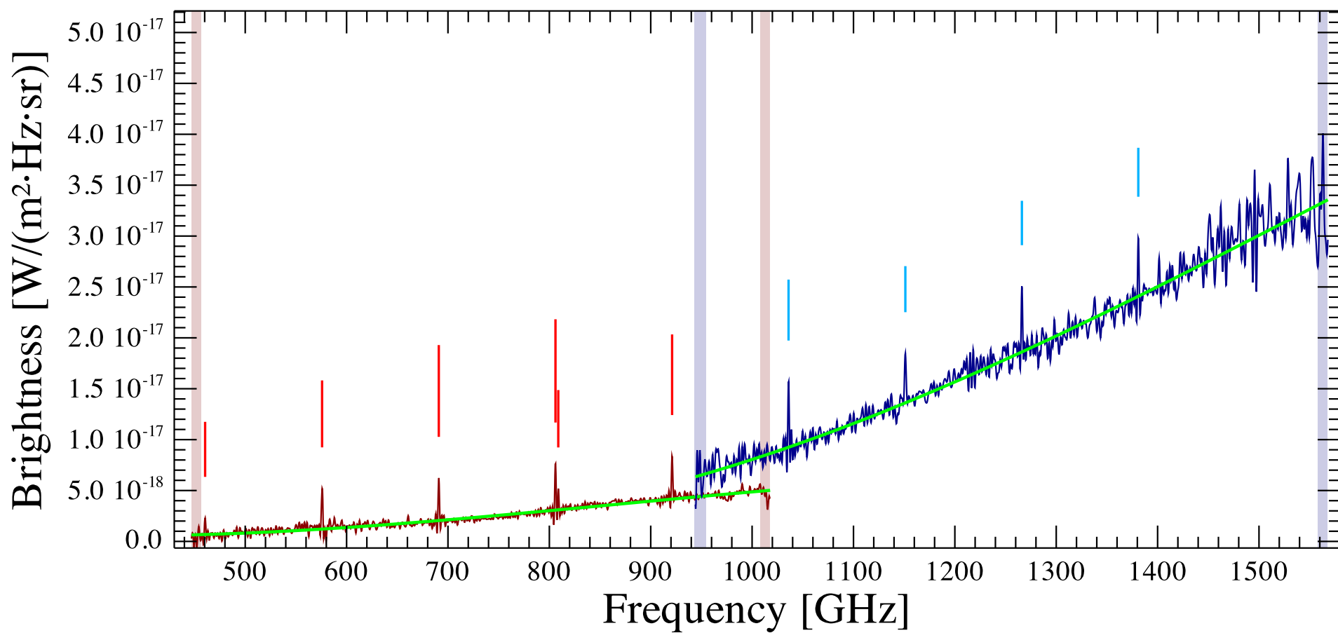
N113-maser Observation ID 1342247763; (6/4)
