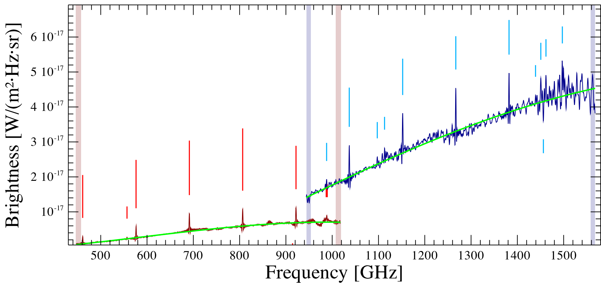
L1157 Observation ID 1342247625; (10/12)
