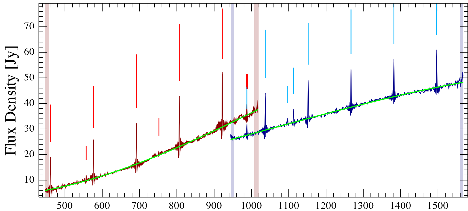
L1157 Observation ID 1342247625; (10/12)
