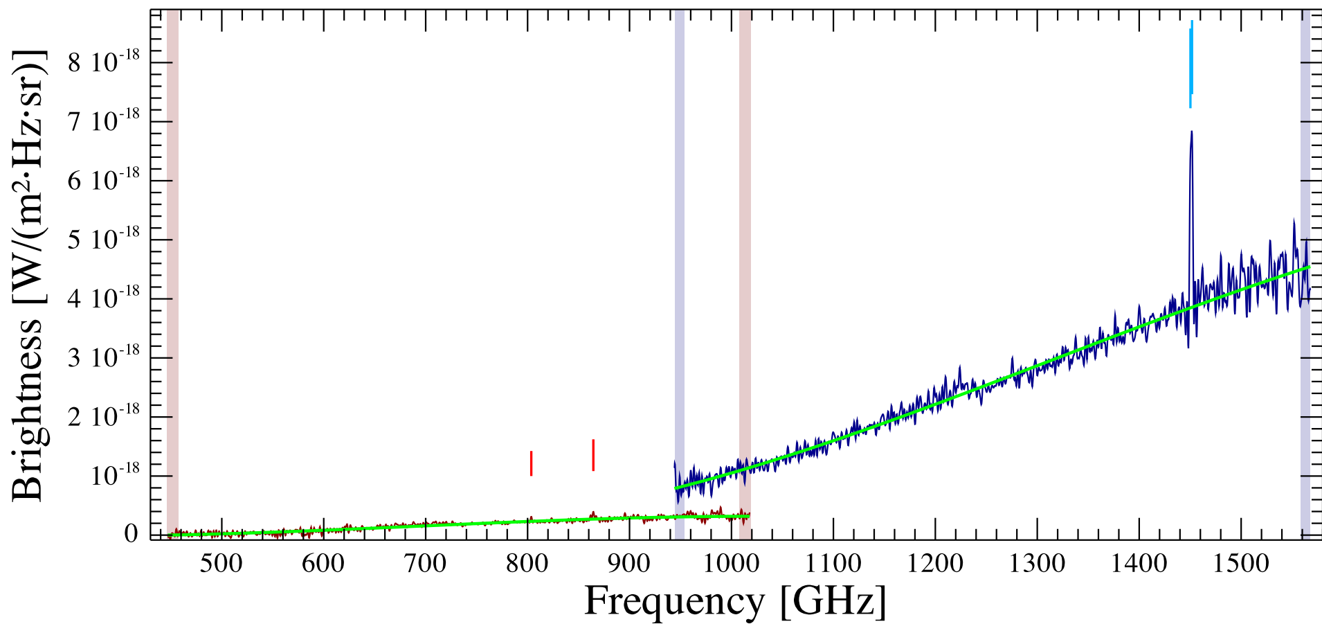
NGC3665 Observation ID 1342247121; (2/2)
