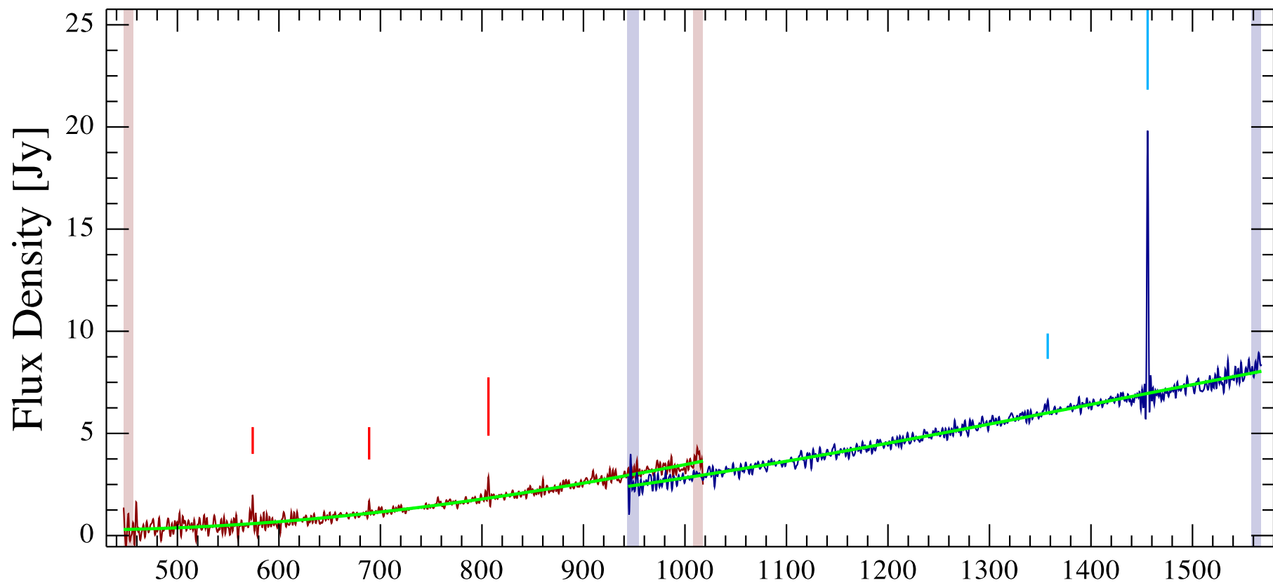
NGC4710 Observation ID 1342247120; (2/1)
