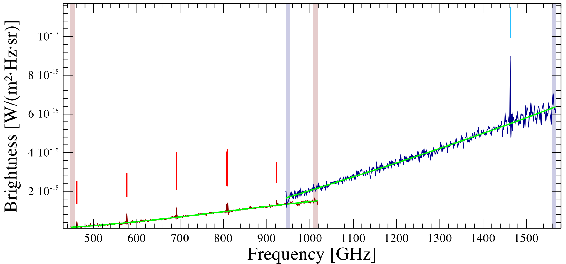
IC10-B11-1 Observation ID 1342246982; (6/1)
