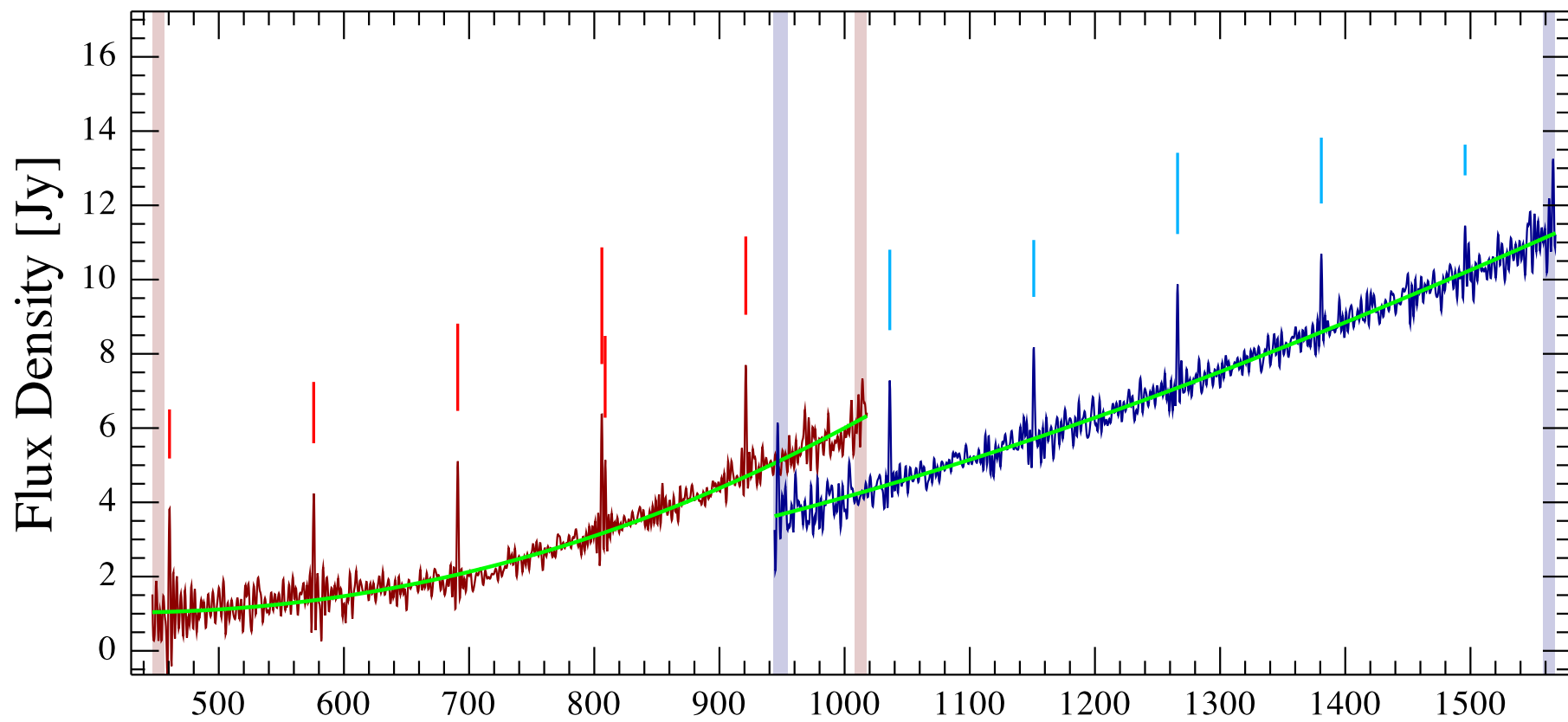
IRAS04514-6931 Observation ID 1342246272; (6/4)
