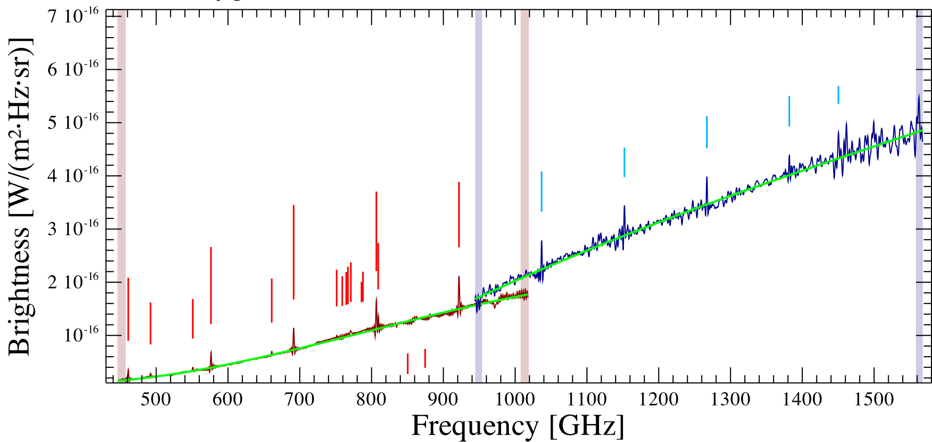
cygn38_sw-1 Observation ID 1342245872; (18/5)
