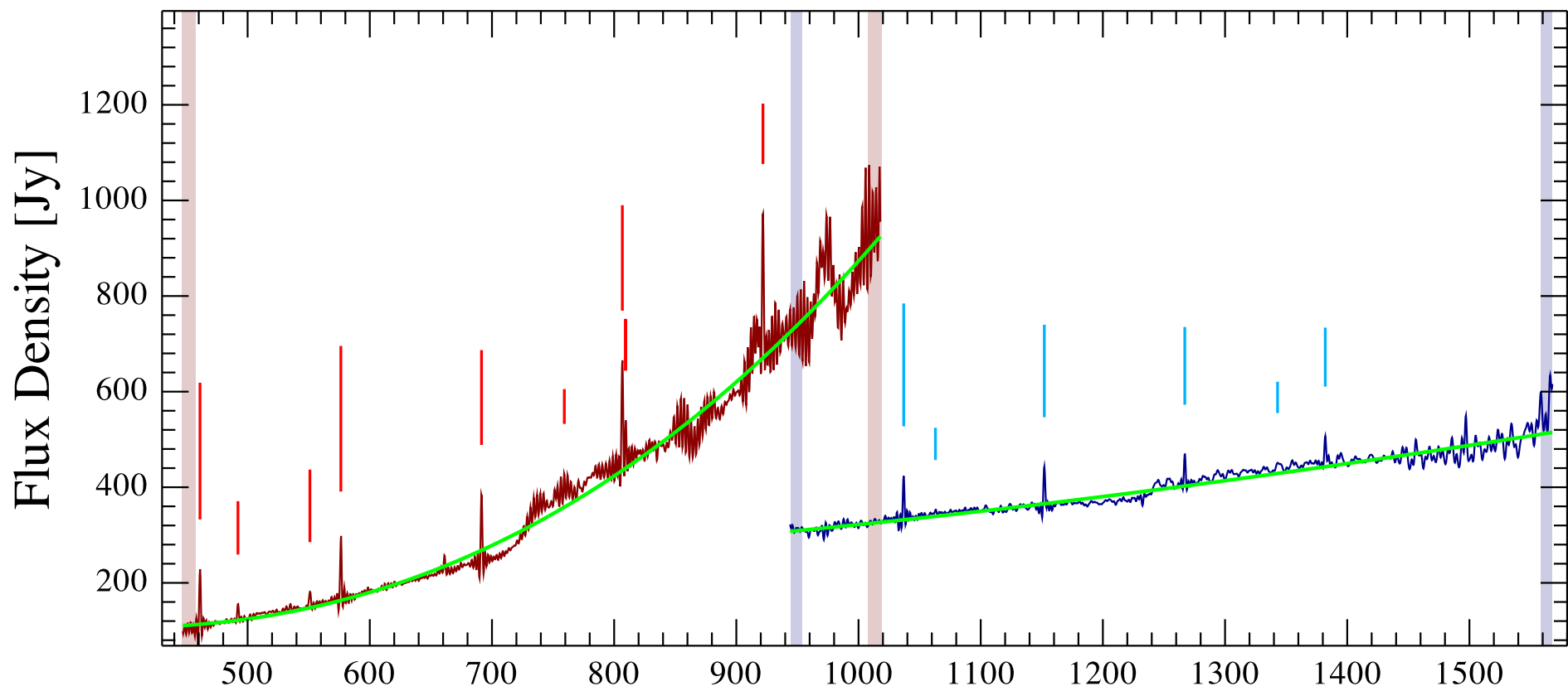
cygn38_sw-1 Observation ID 1342245872; (18/5)
