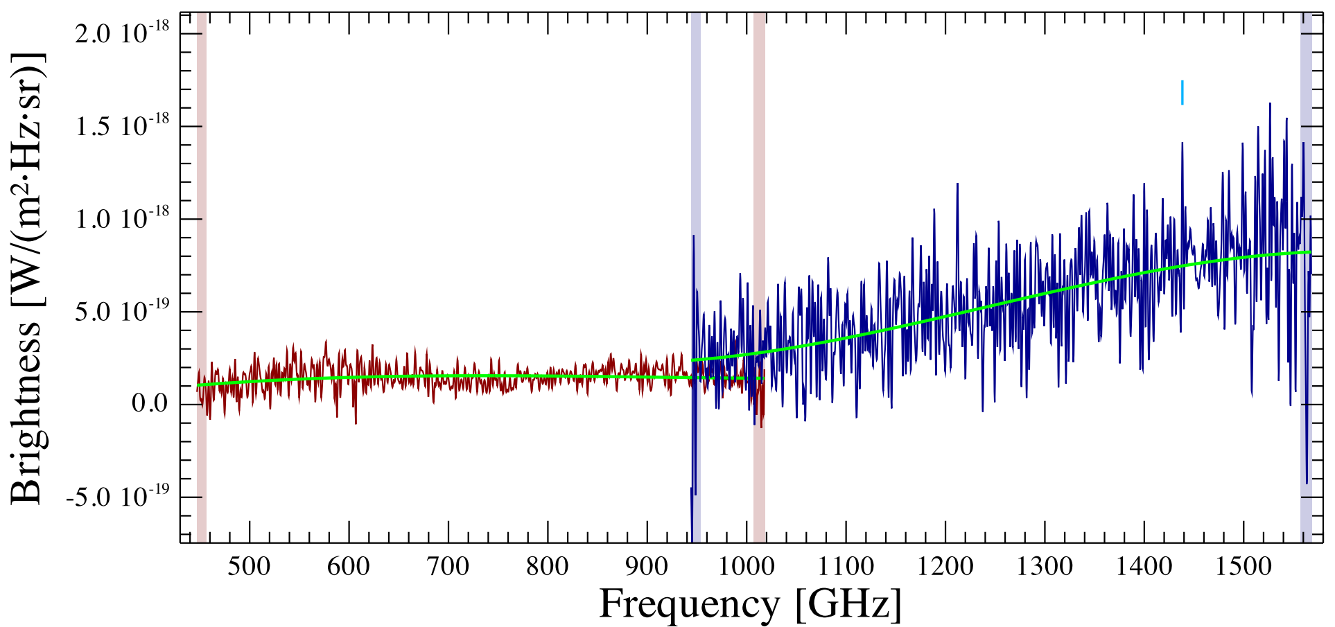
NGC 3242 Observation ID 1342245847; (0/1)
