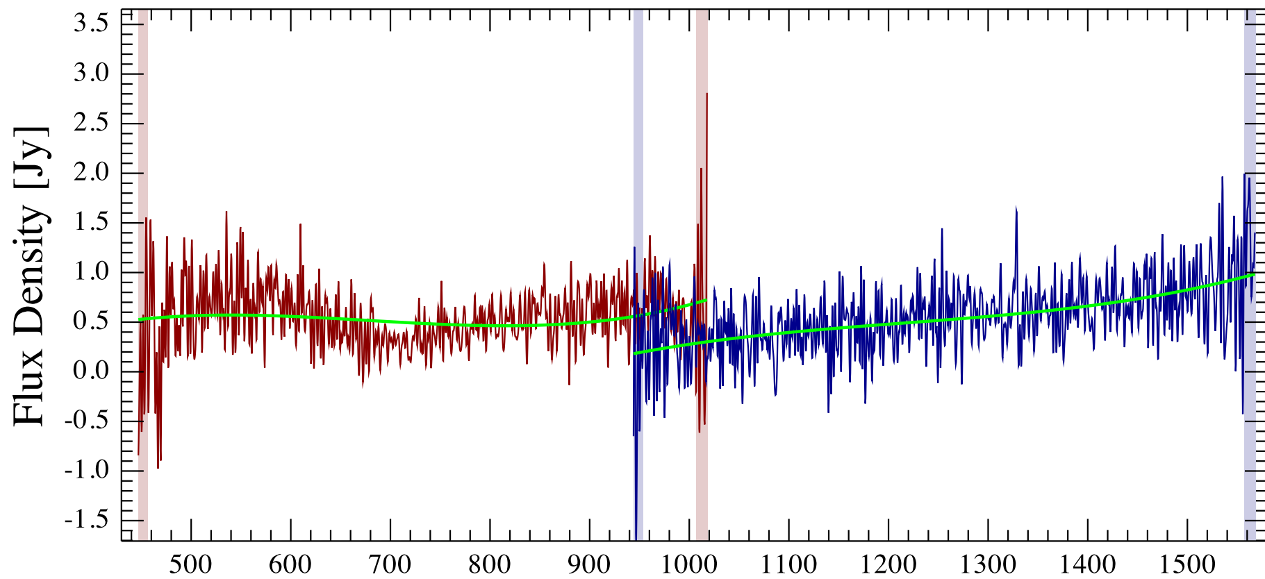
NGC 3242 S Flier Observation ID 1342245846; (0/0)
