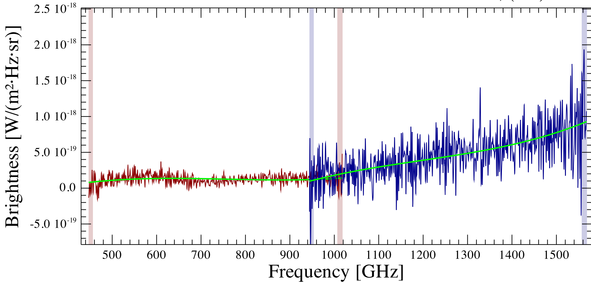
NGC 3242 S Flier Observation ID 1342245846; (0/0)
