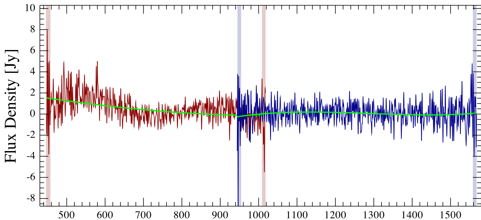
NGC 3242 OFF Observation ID 1342245845; (0/0)
