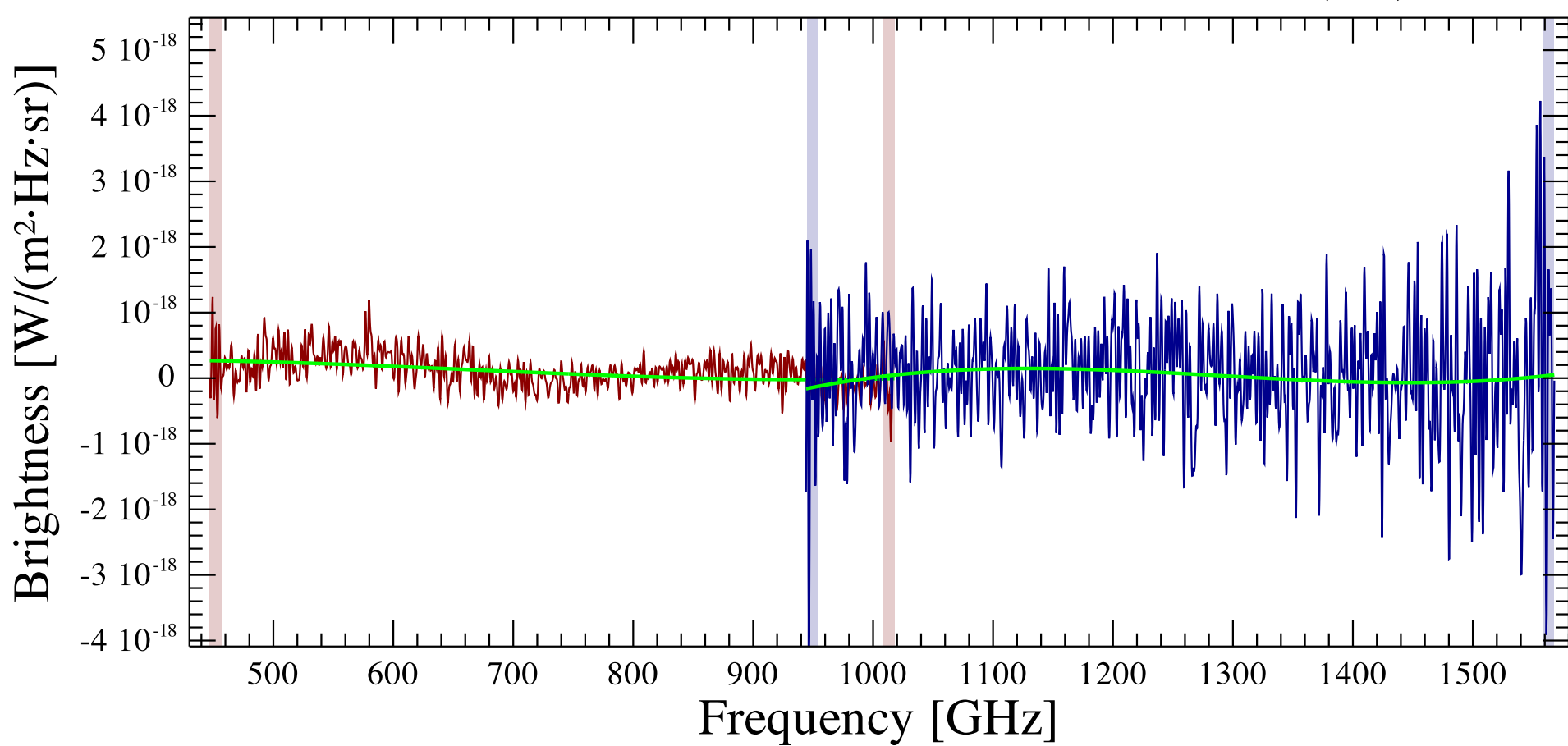
NGC 3242 OFF Observation ID 1342245845; (0/0)
