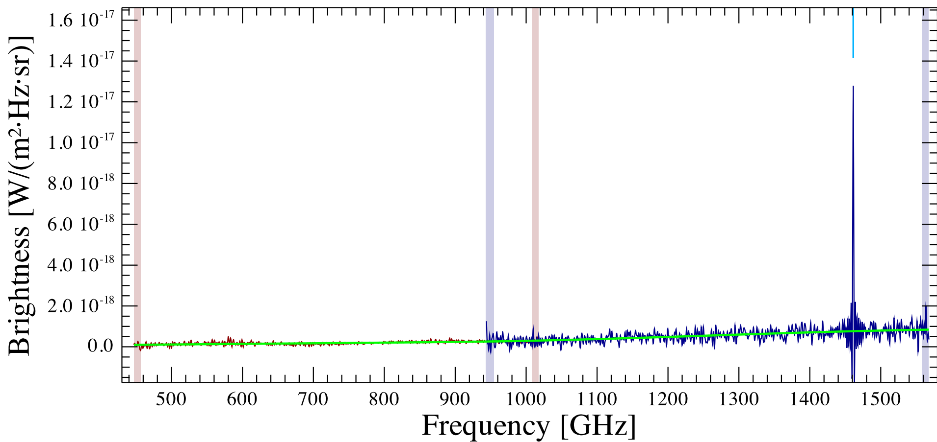
NGC 40 W Rim Observation ID 1342245122; (0/1)
