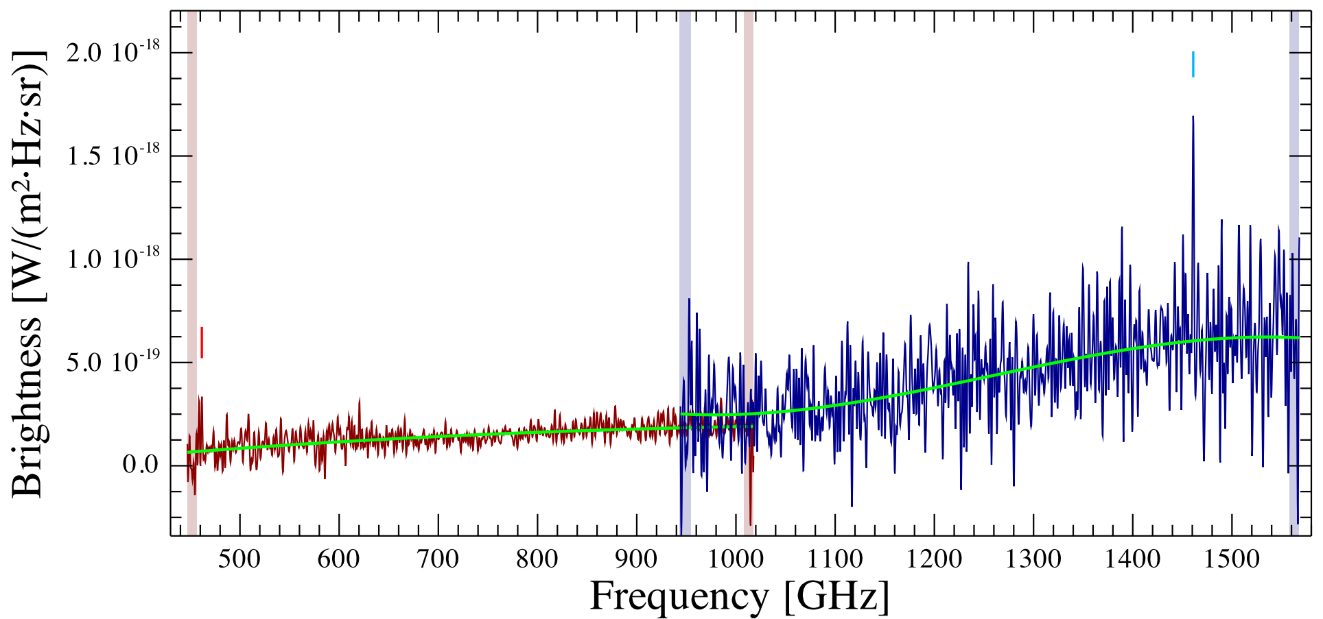
NGC 2392 Observation ID 1342245121; (1/1)
