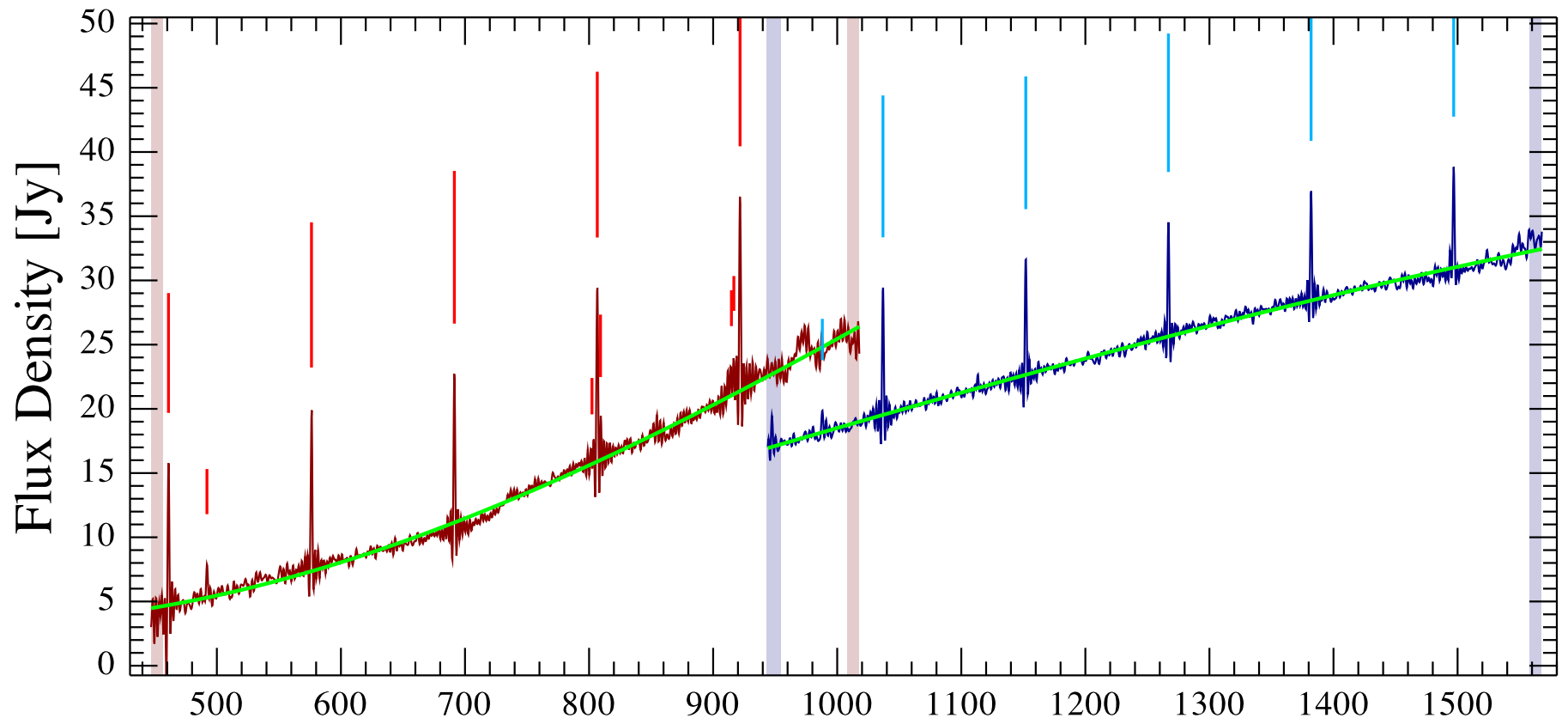
L723 MM Observation ID 1342245094; (7/10)
