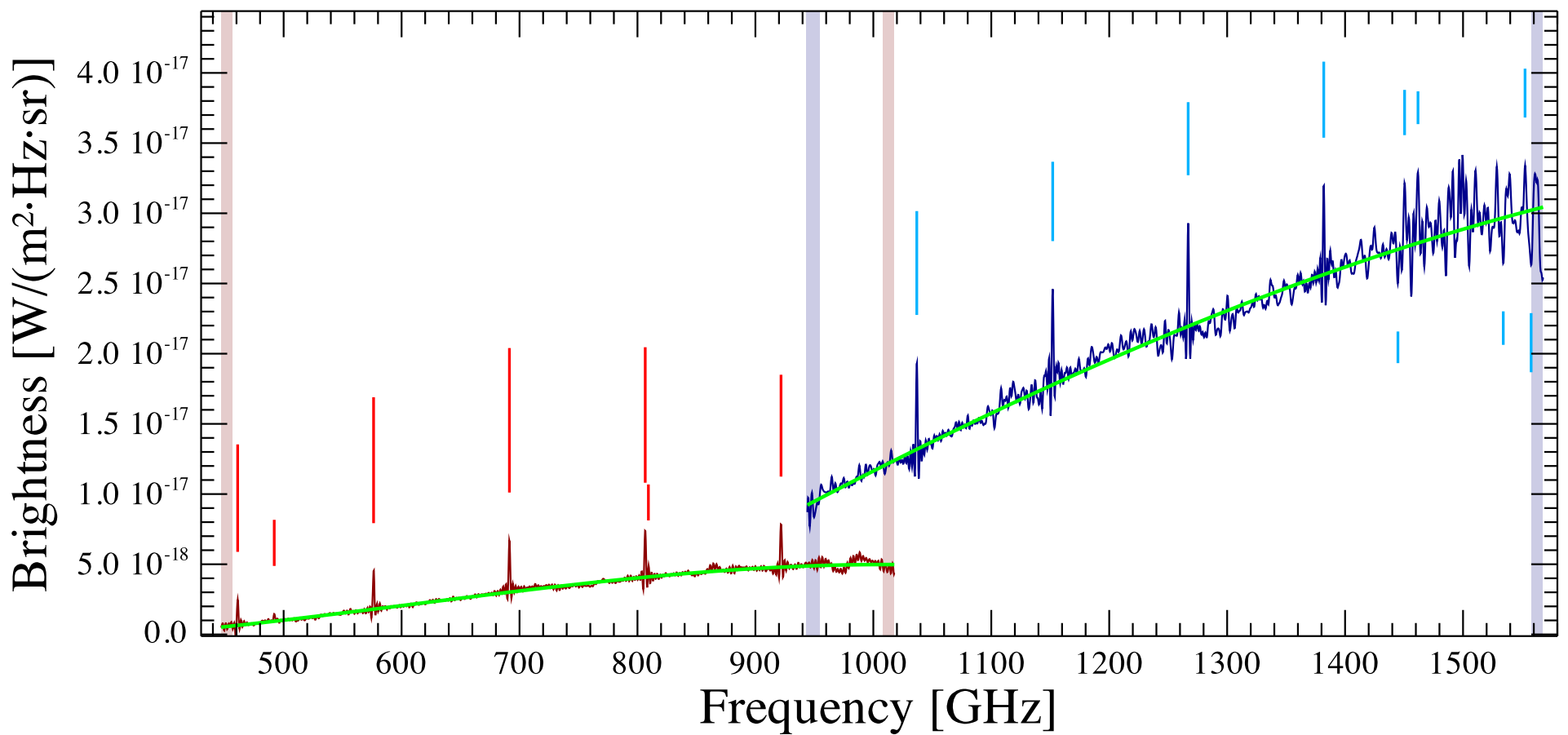
L723 MM Observation ID 1342245094; (7/10)
