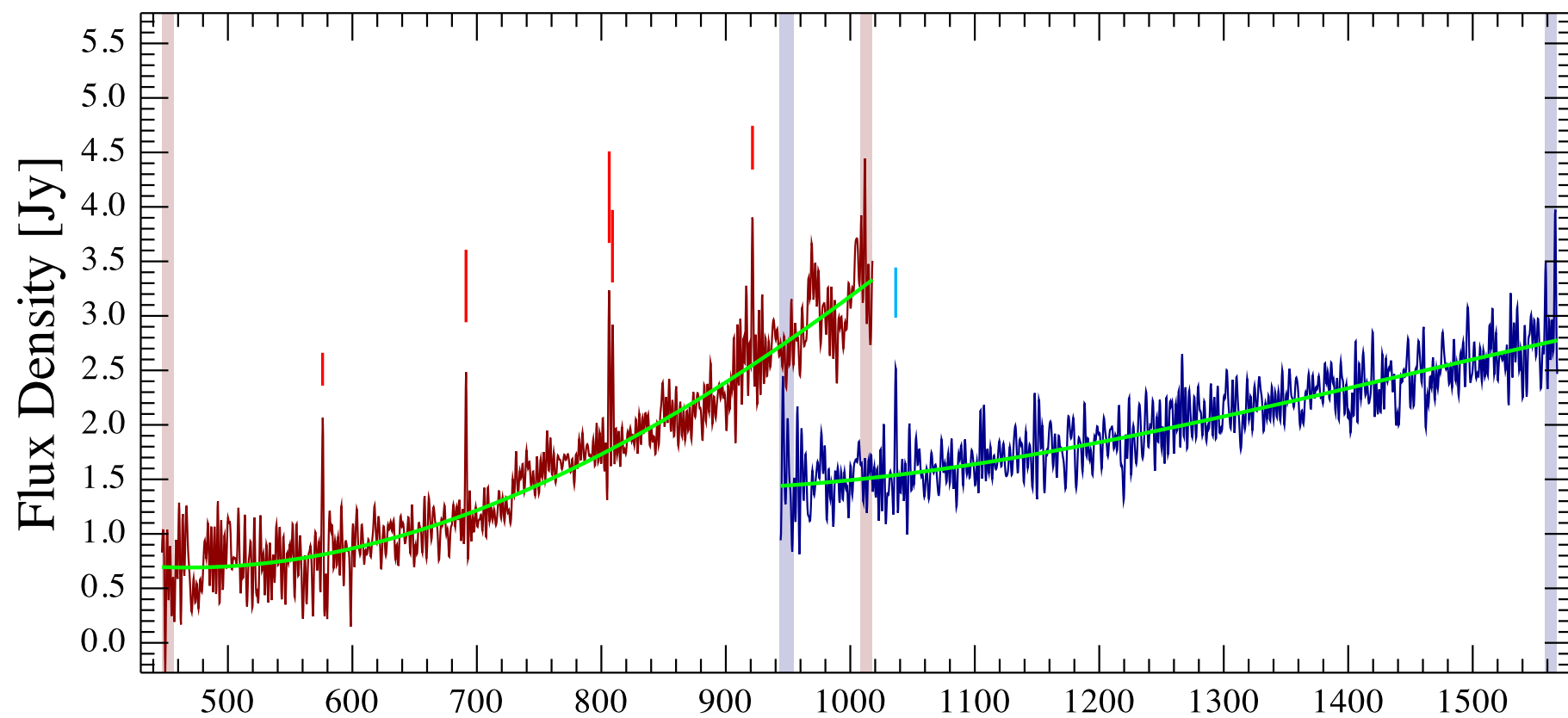
IRAS00464-7322 Observation ID 1342245092; (5/1)
