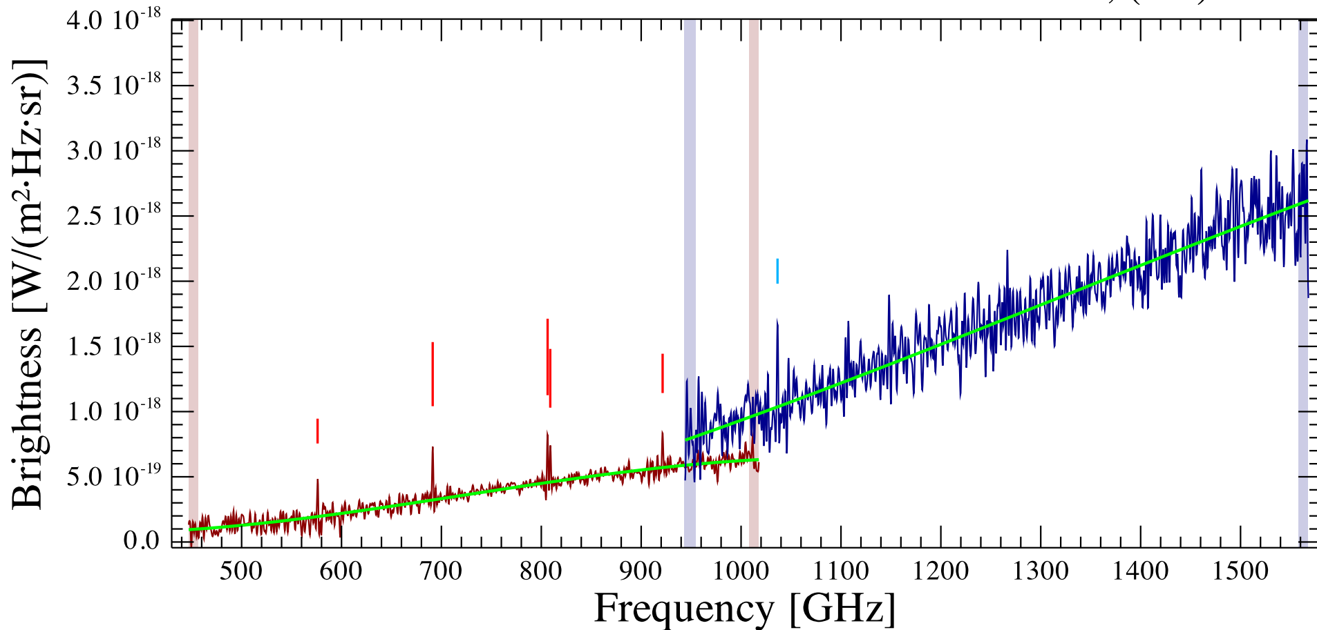
IRAS00464-7322 Observation ID 1342245092; (5/1)
