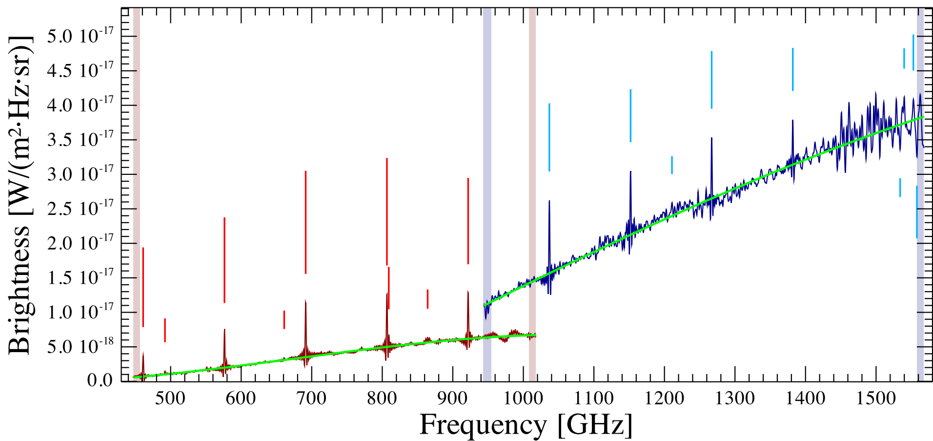
HH 46 Observation ID 1342245084; (9/9)
