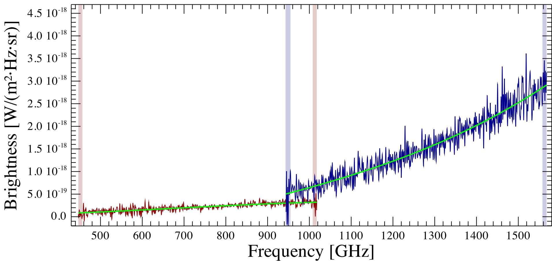
NGC 7009 Observation ID 1342245079; (0/0)
