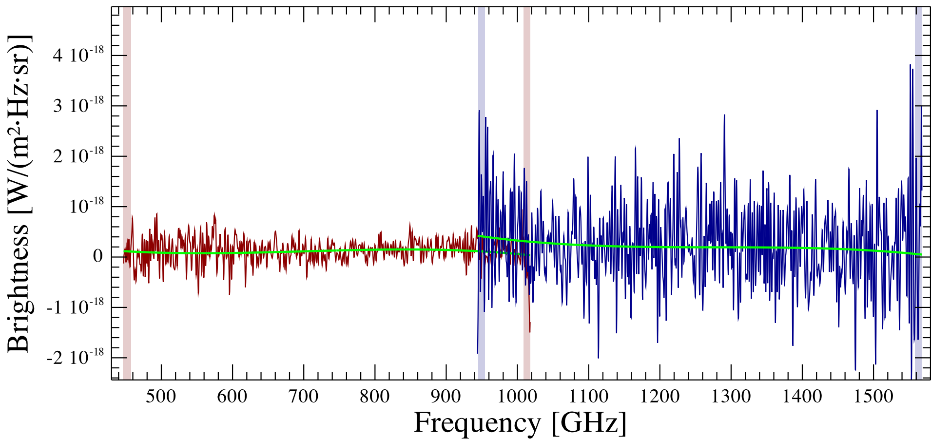
NGC 40 OFF Observation ID 1342243641; (0/0)
