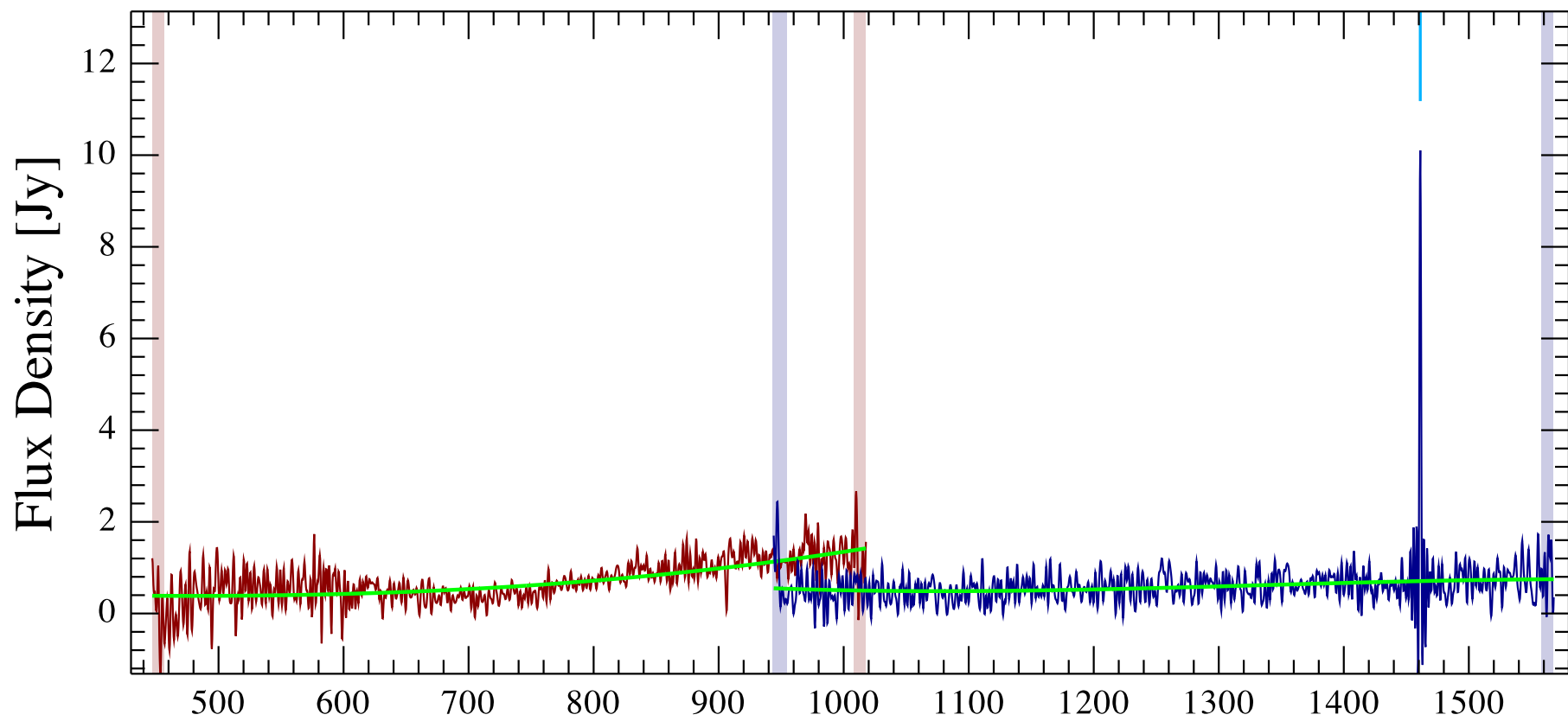
NGC 40 Observation ID 1342243640; (0/1)
