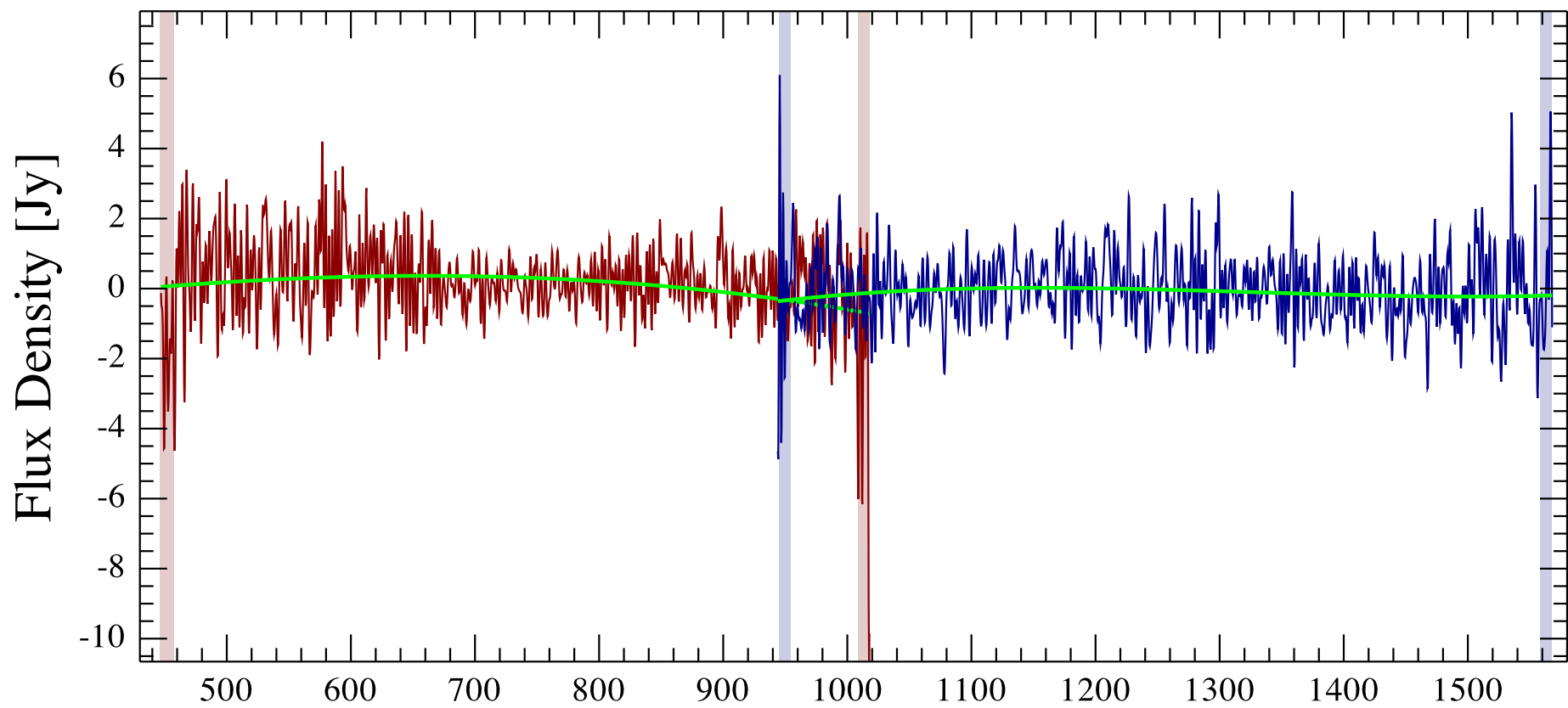
NGC 6720 OFF Observation ID 1342243618; (0/0)
