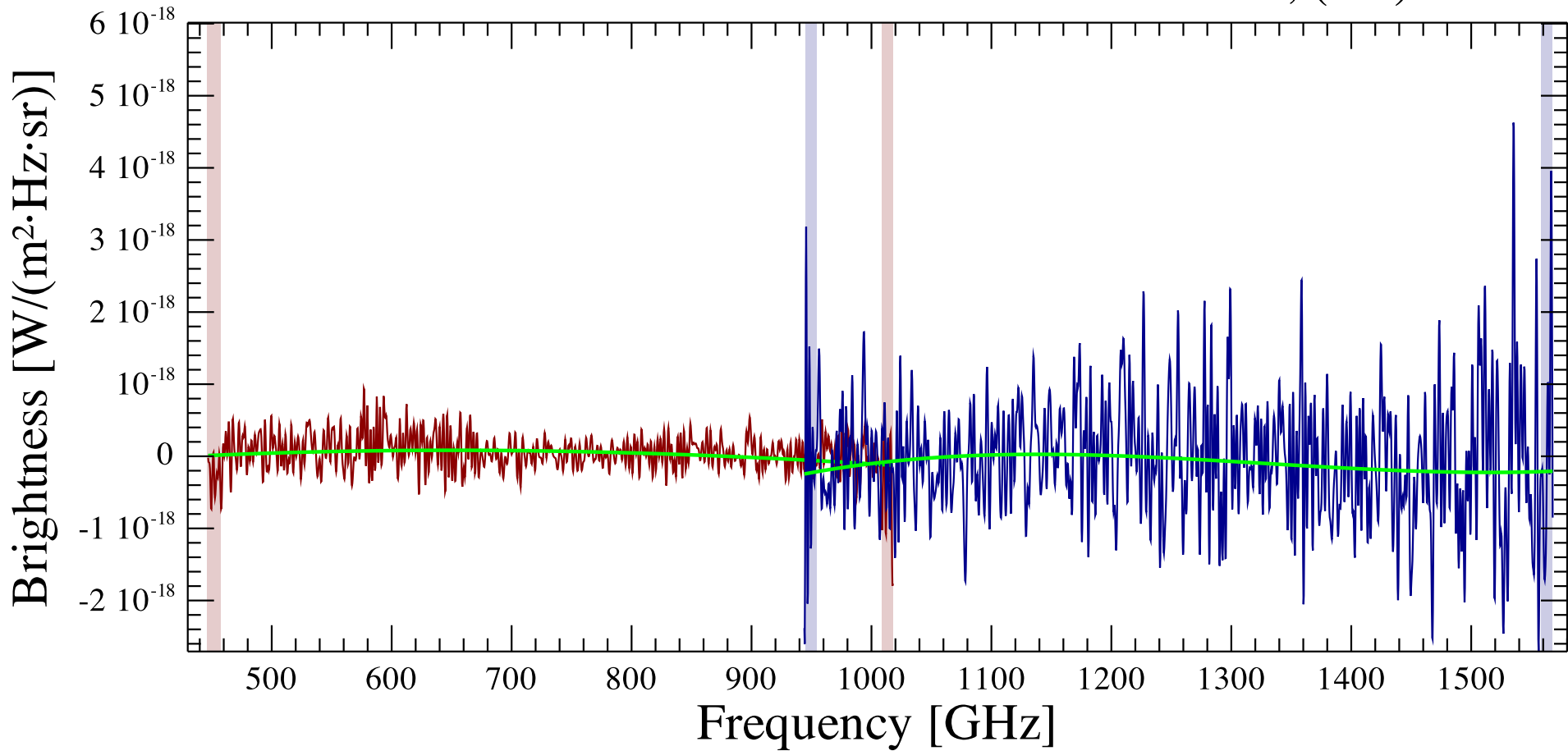
NGC 6720 OFF Observation ID 1342243618; (0/0)
