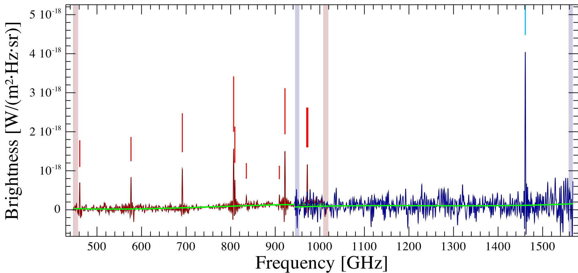
NGC 6720 Observation ID 1342243616; (9/1)
