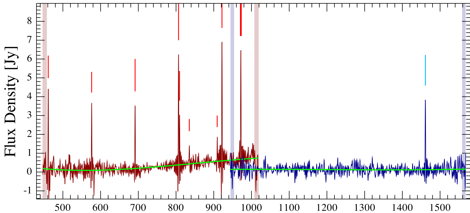
NGC 6720 Observation ID 1342243616; (9/1)
