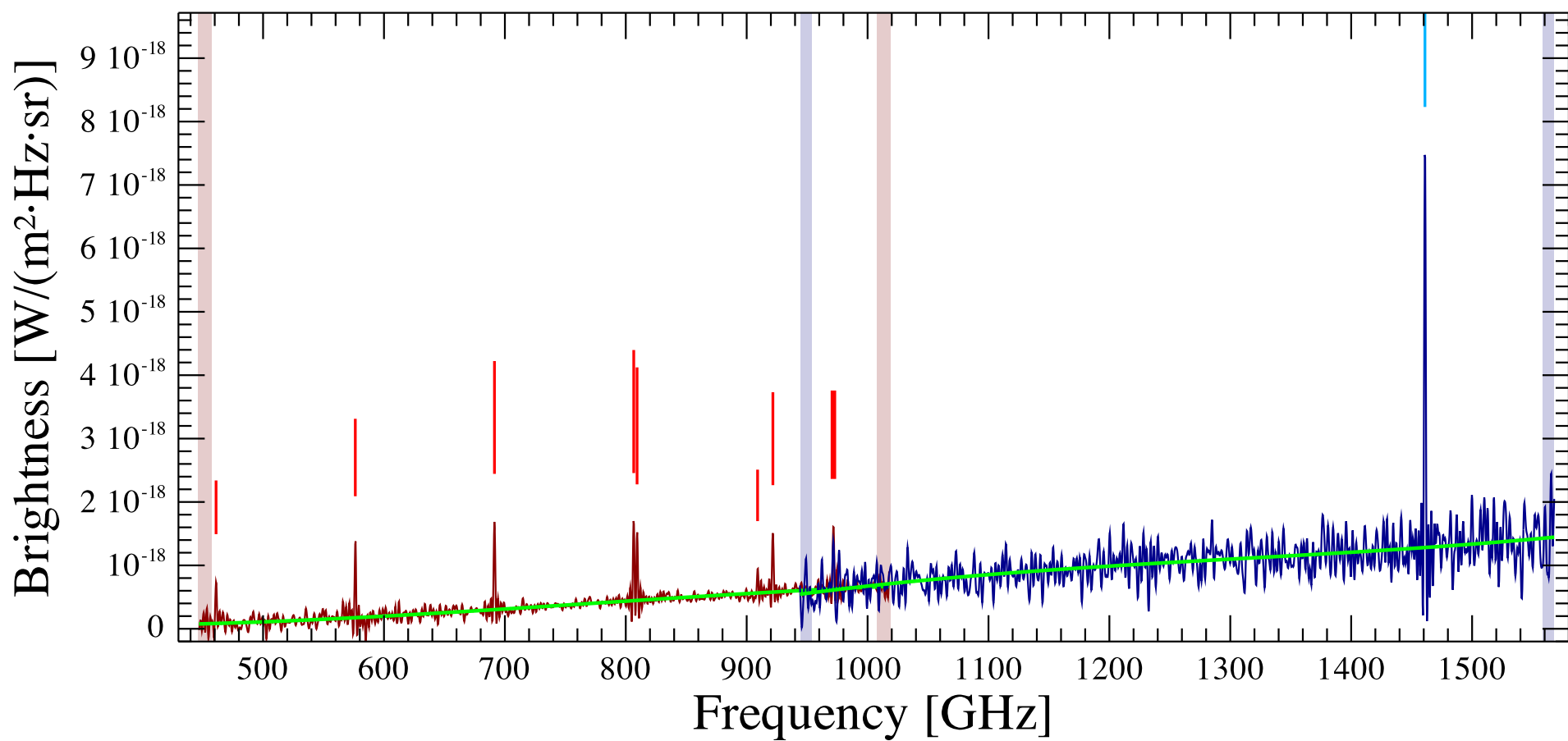
NGC 6781 Observation ID 1342243612; (8/1)
