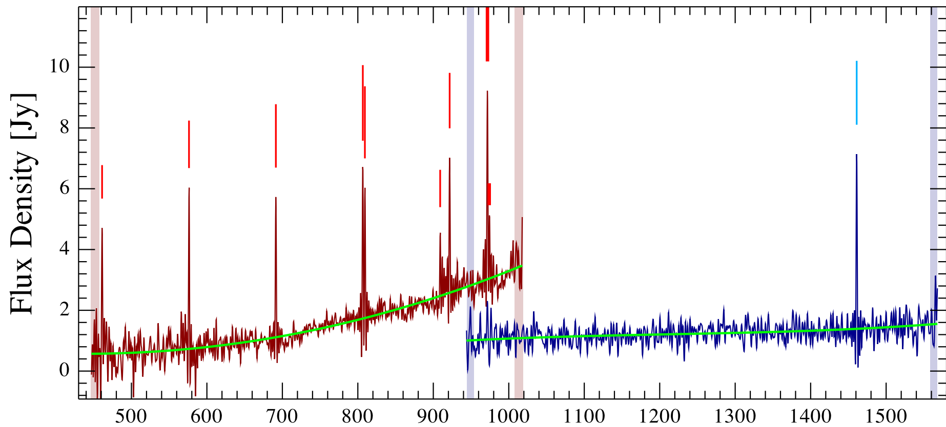
NGC 6781 Observation ID 1342243612; (8/1)
