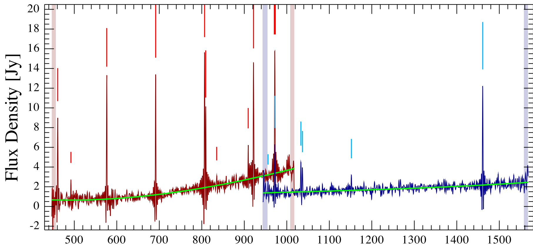
NGC 6781 Rim Observation ID 1342243611; (10/6)
