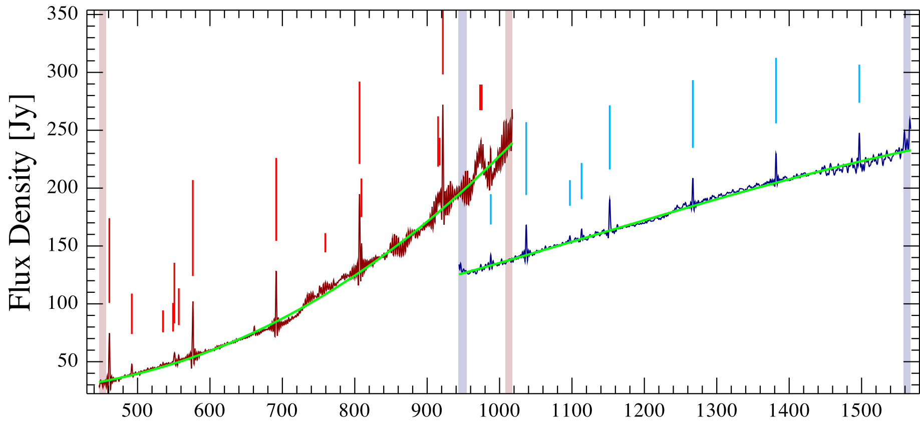
HOPS 87 Observation ID 1342242623; (16/8)
