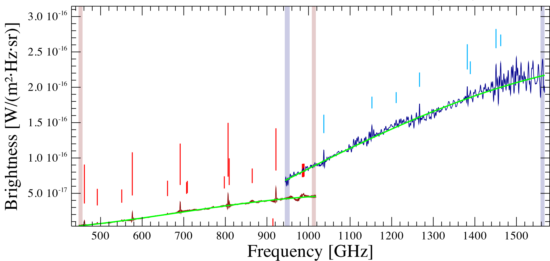
HOPS 87 Observation ID 1342242623; (16/8)
