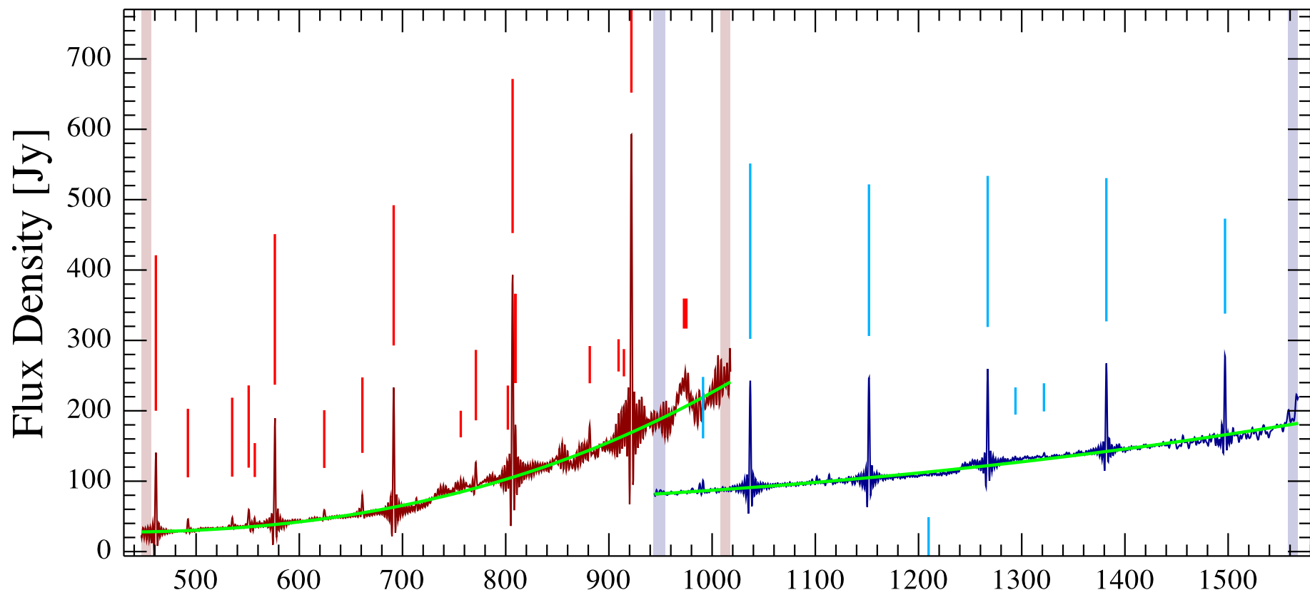
RCrA-IRS7B Observation ID 1342242620; (18/13)
