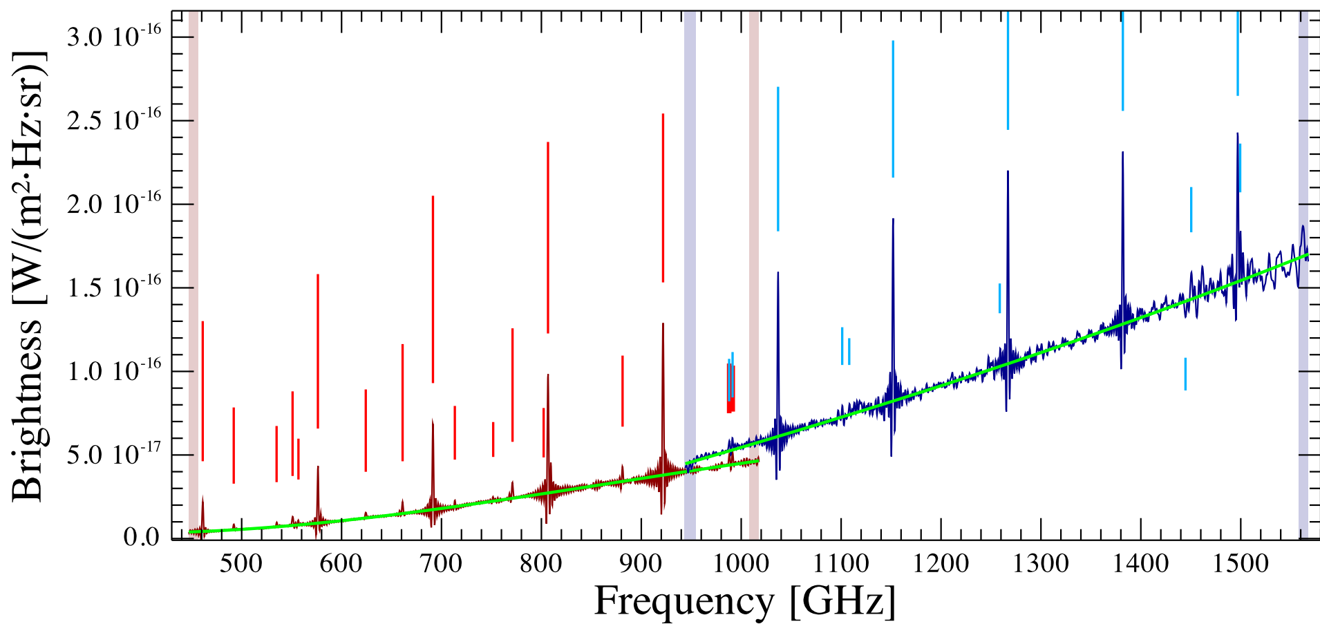
RCrA-IRS7B Observation ID 1342242620; (18/13)
