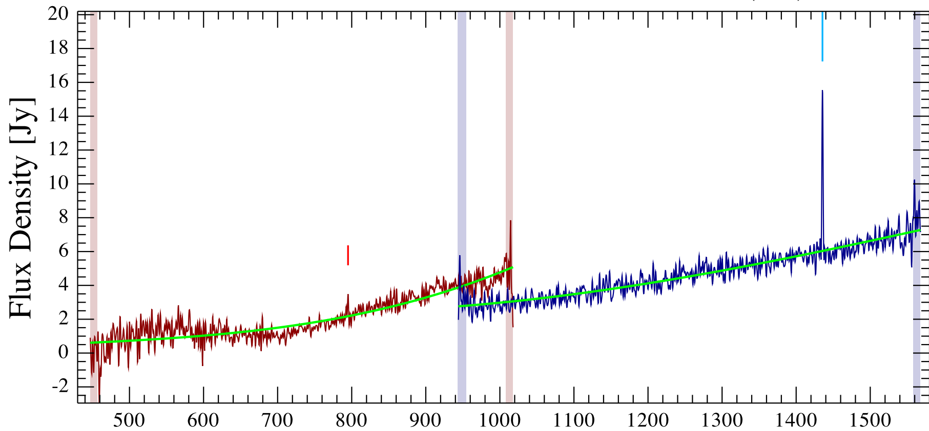
UGC02982 Observation ID 1342240021; (1/1)
