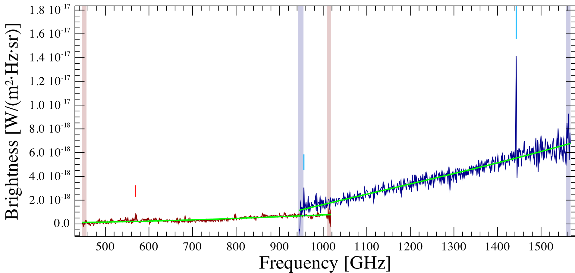
NGC5990 Observation ID 1342240016; (1/2)
