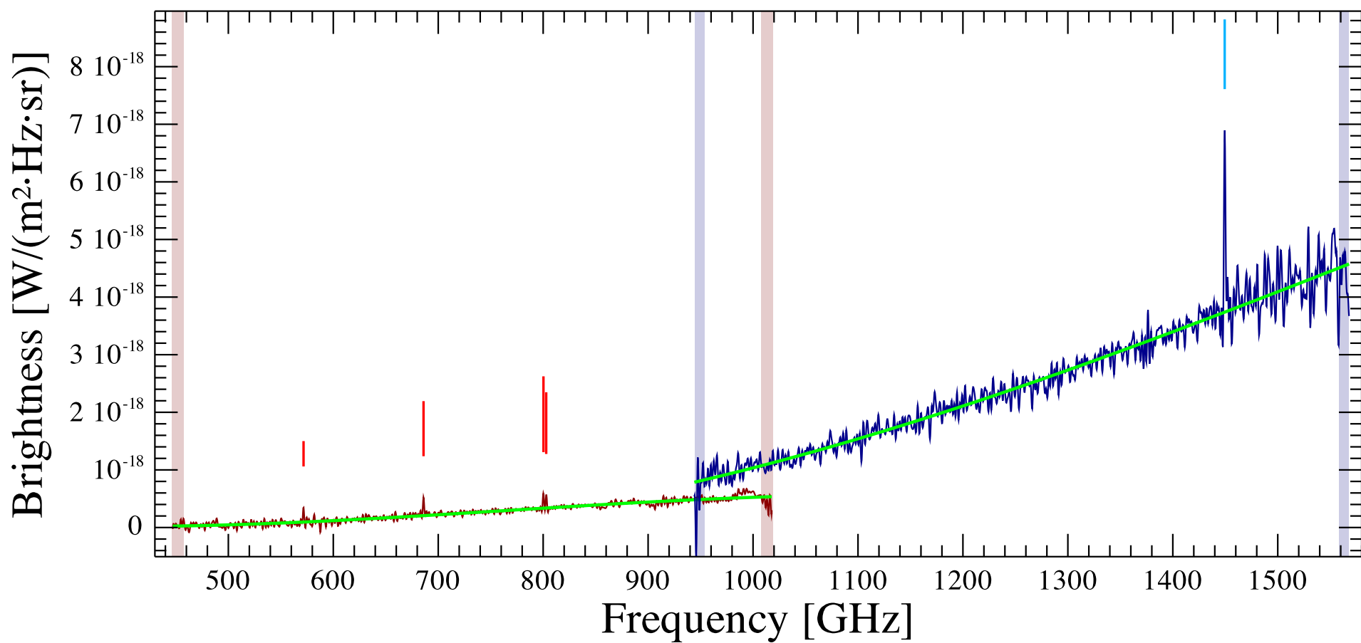
NGC1222 Observation ID 1342239354; (4/1)
