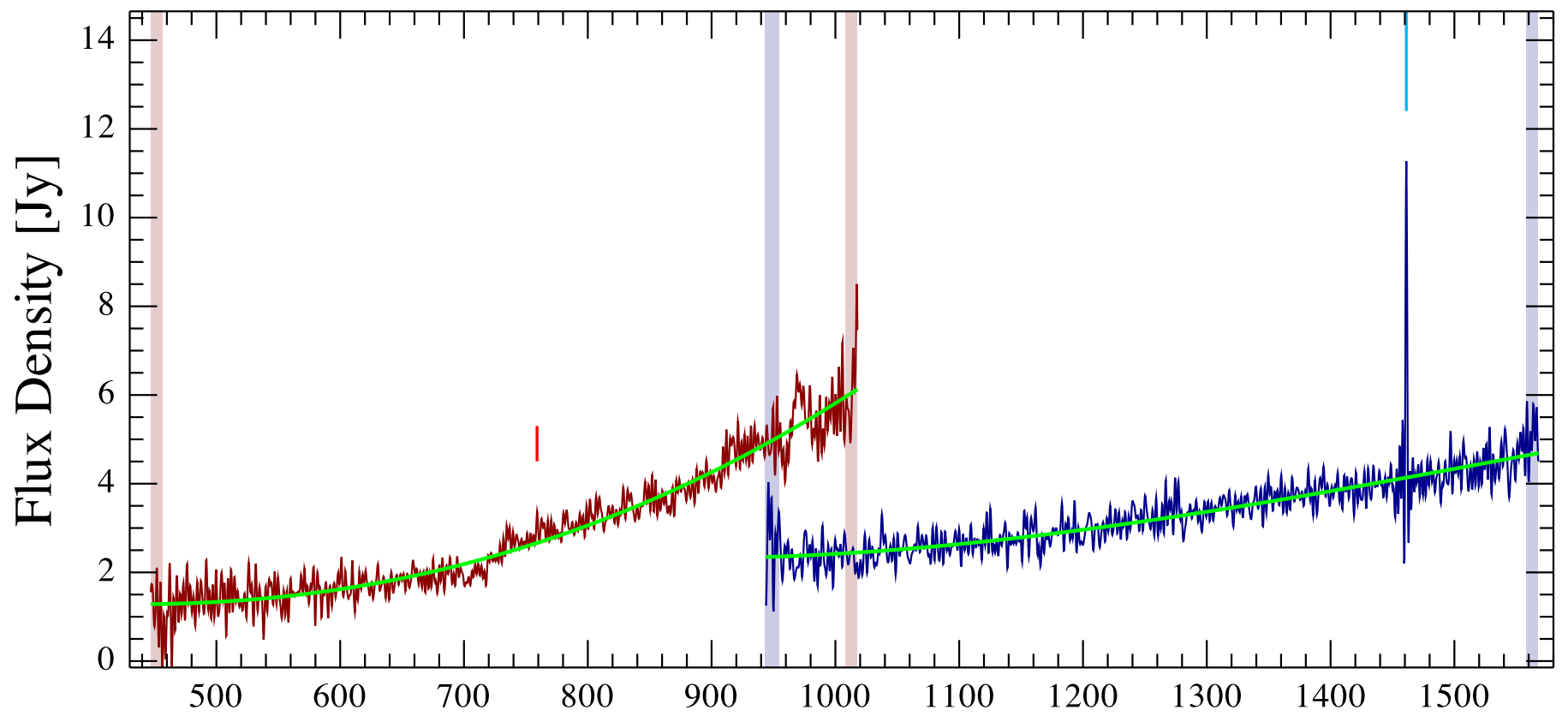
NGC 7026 Observation ID 1342239347; (0/1)
