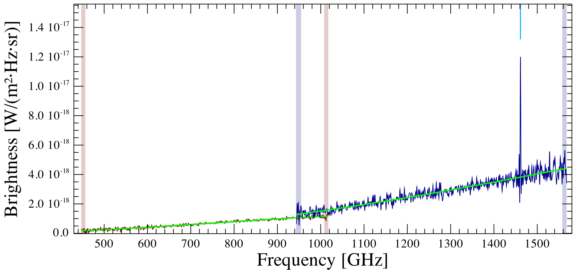
NGC 7026 Observation ID 1342239347; (0/1)
