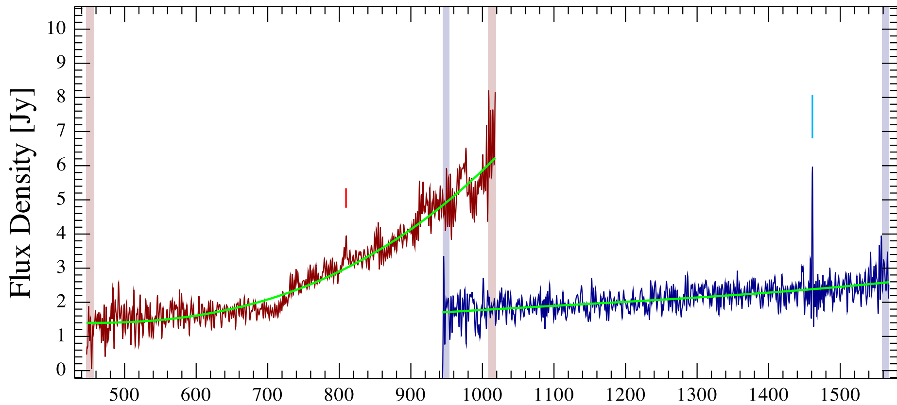
NGC 7026 N Lobe Observation ID 1342239346; (1/1)
