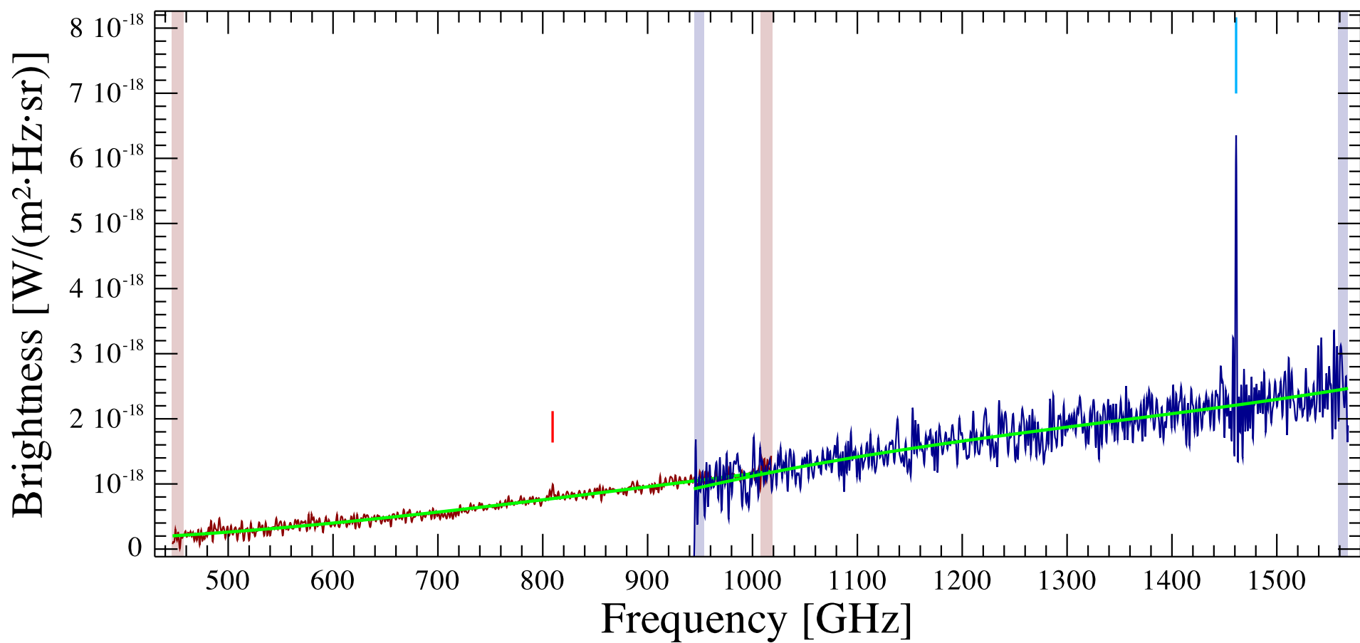
NGC 7026 N Lobe Observation ID 1342239346; (1/1)
