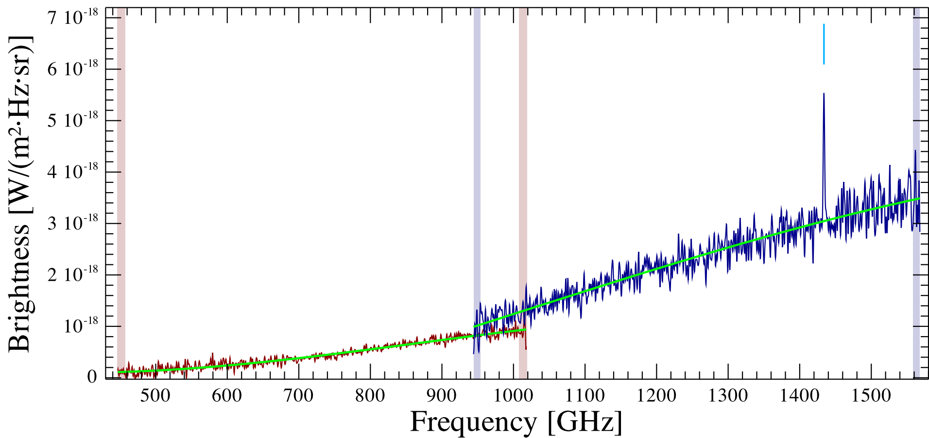
NGC0958 Observation ID 1342239339; (0/1)
