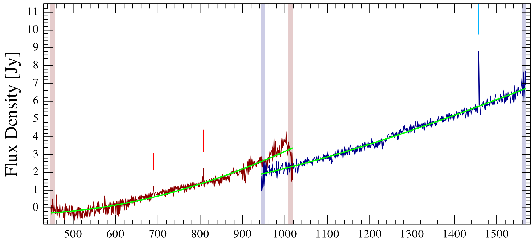
NGC5866 Observation ID 1342238708; (2/1)
