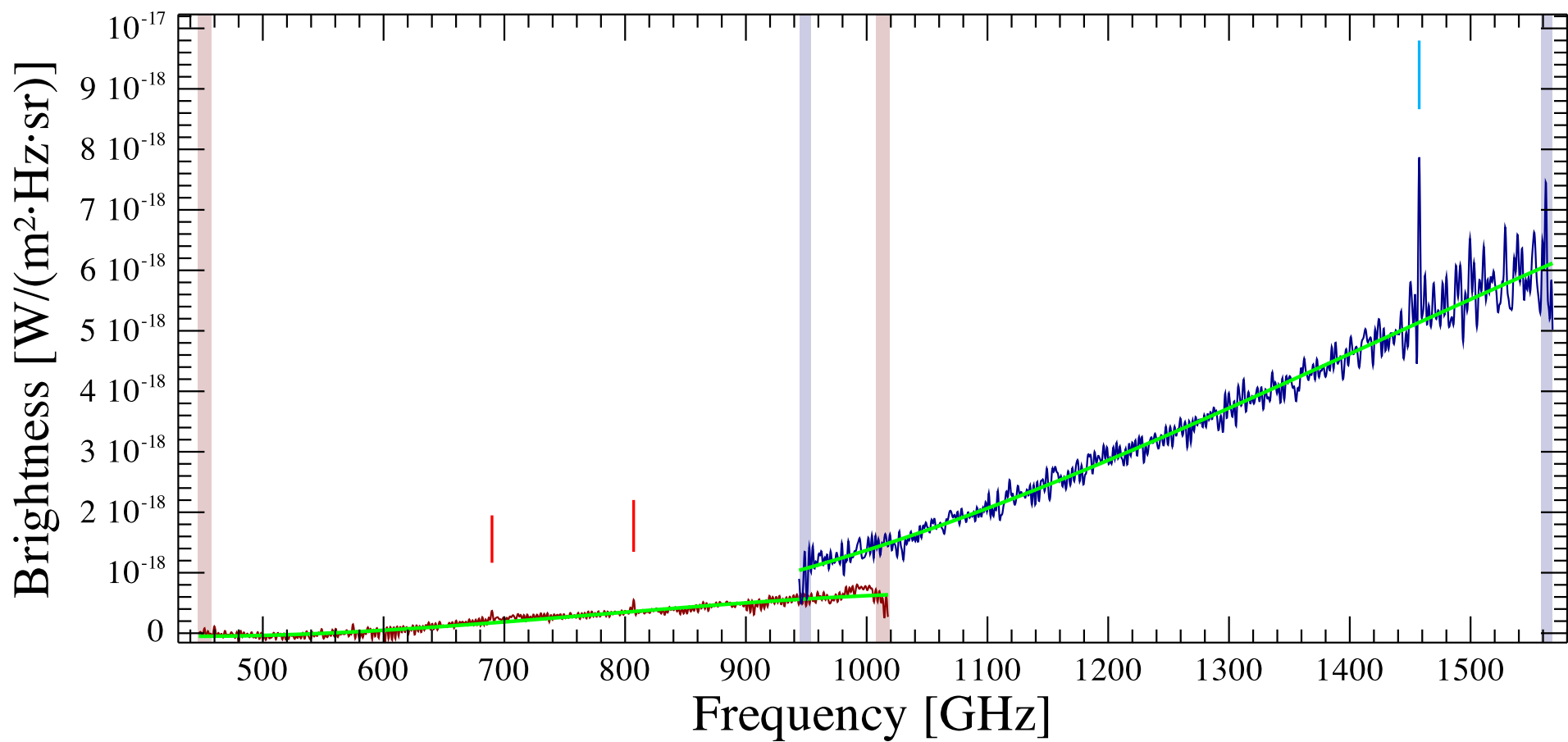
NGC5866 Observation ID 1342238708; (2/1)
