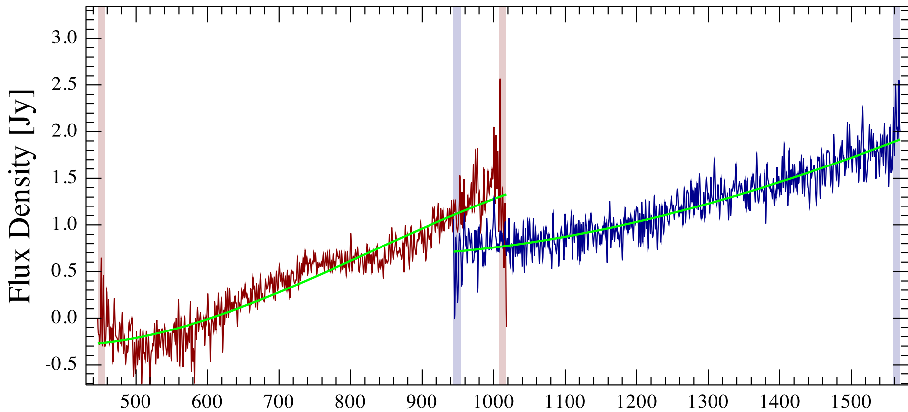
IRAS 03521+0028 Observation ID 1342238704; (0/0)
