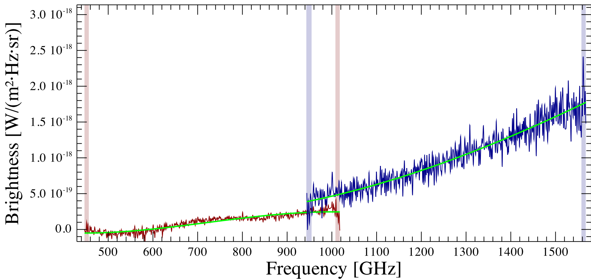
IRAS 03521+0028 Observation ID 1342238704; (0/0)
