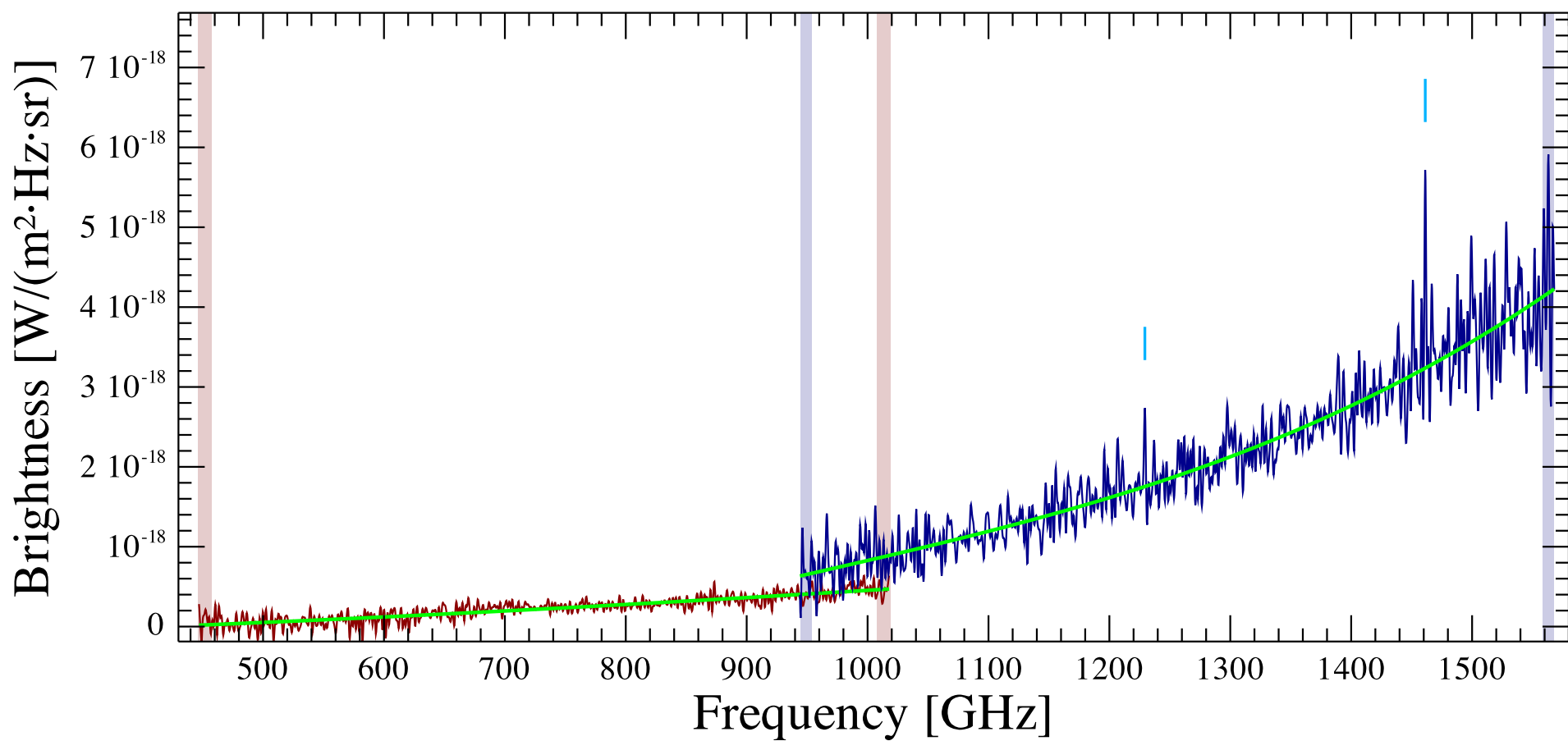
NGC 6543 Observation ID 1342237028; (0/2)
