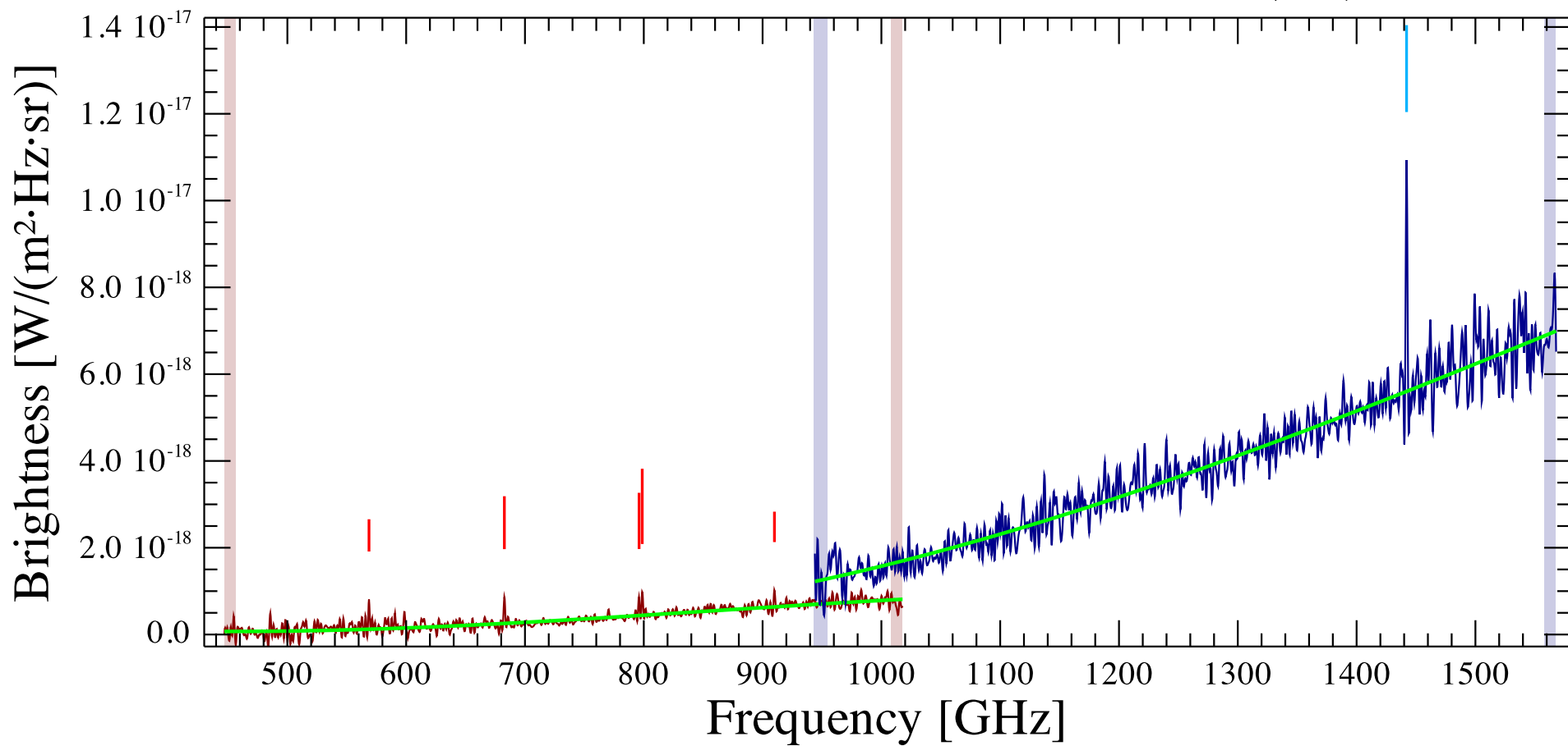
NGC6701 Observation ID 1342231994; (5/1)
