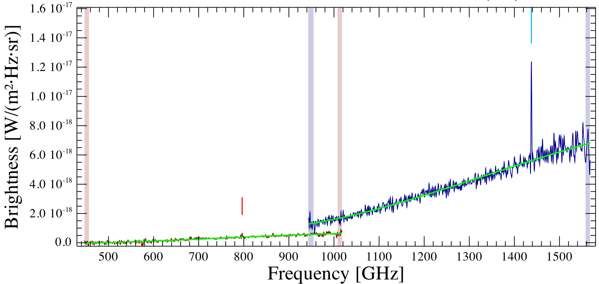
UGC11041 Observation ID 1342231061; (1/1)
