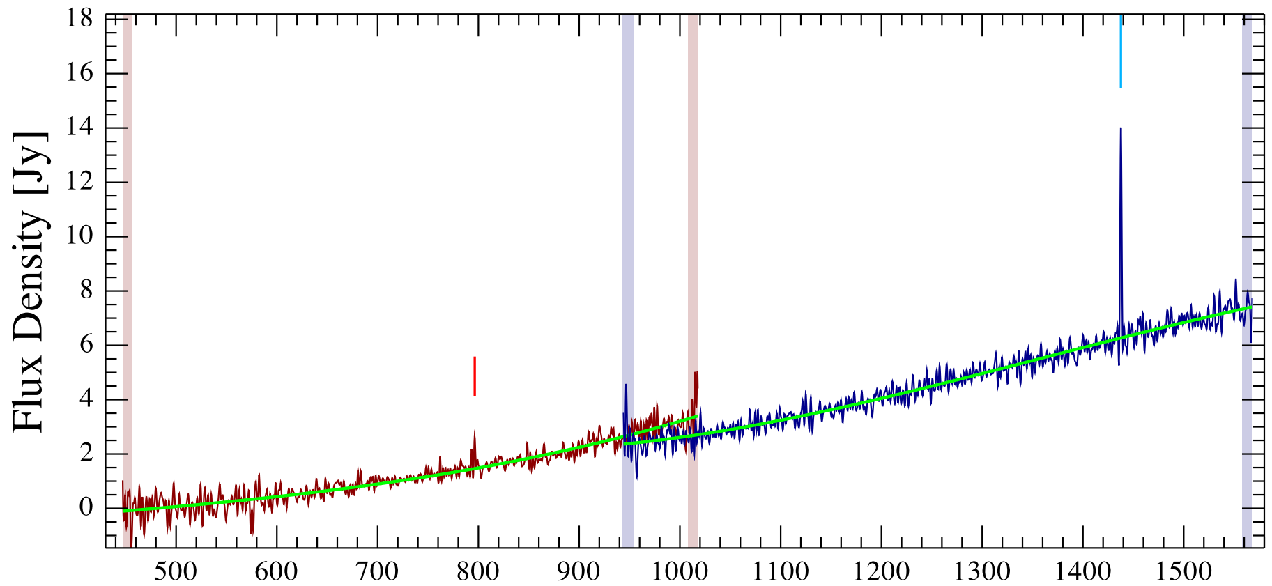
UGC11041 Observation ID 1342231061; (1/1)
