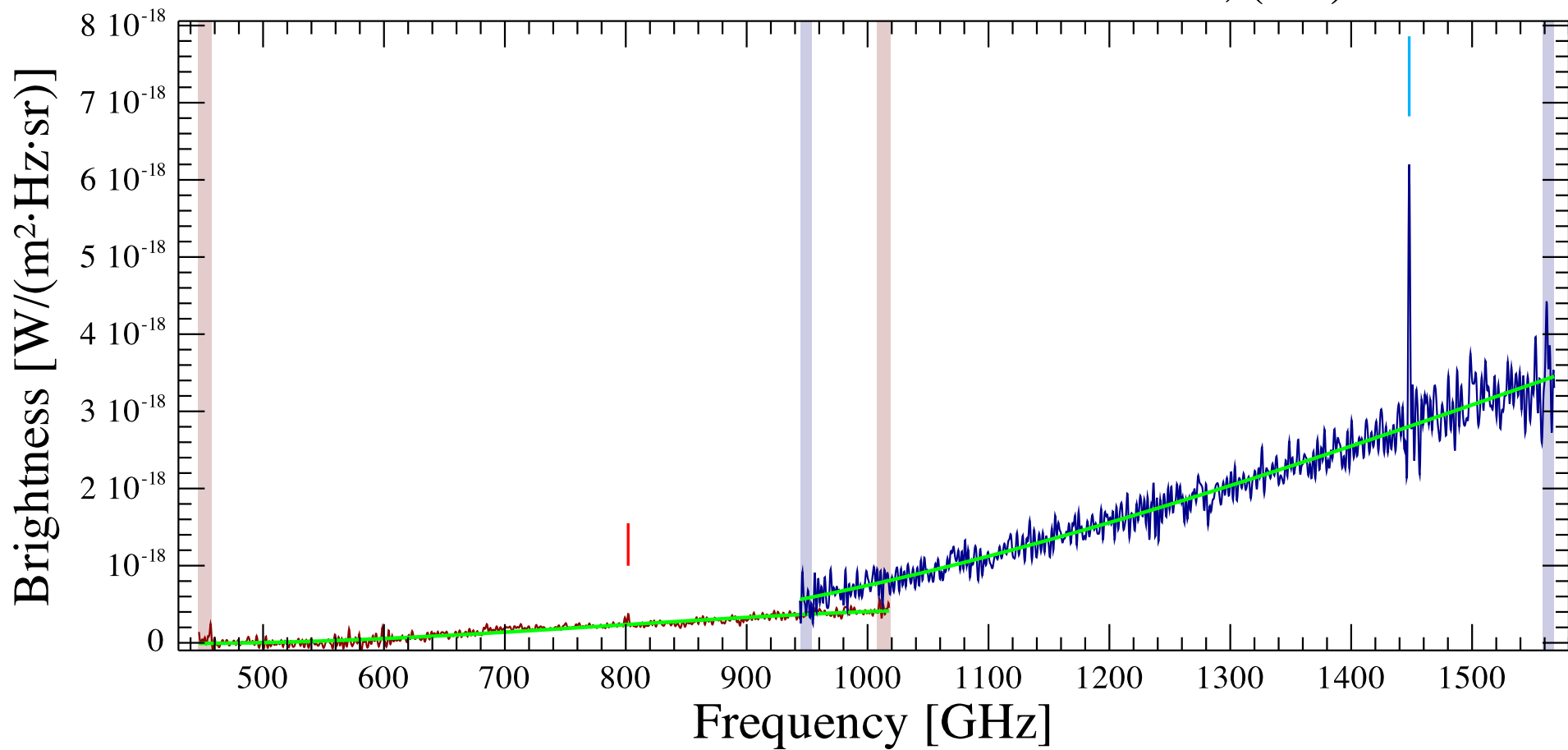
NGC2764 Observation ID 1342231057; (1/1)
