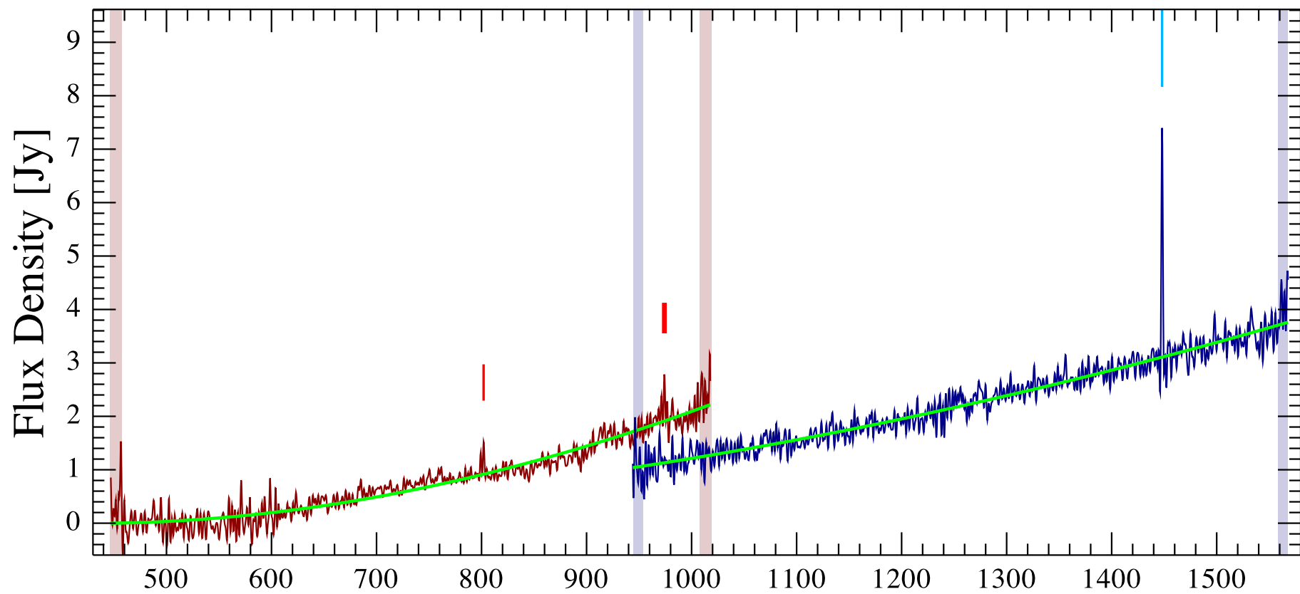
NGC2764 Observation ID 1342231057; (1/1)
