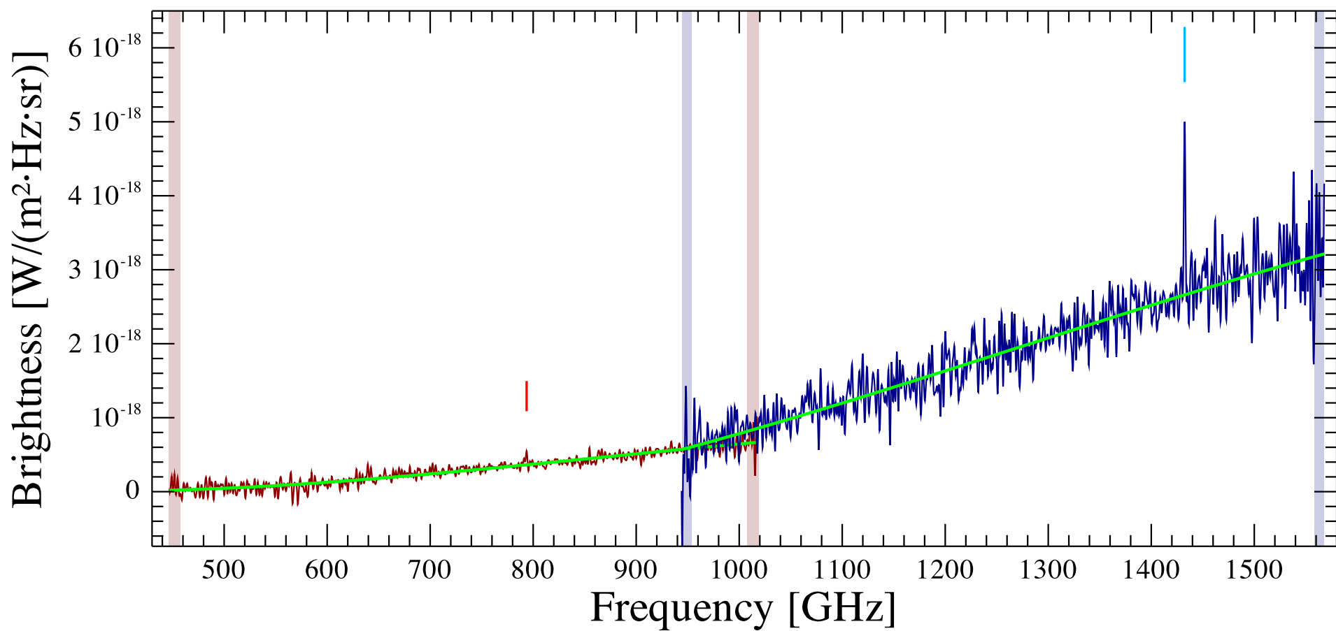
NGC6926 Observation ID 1342231050; (1/1)
