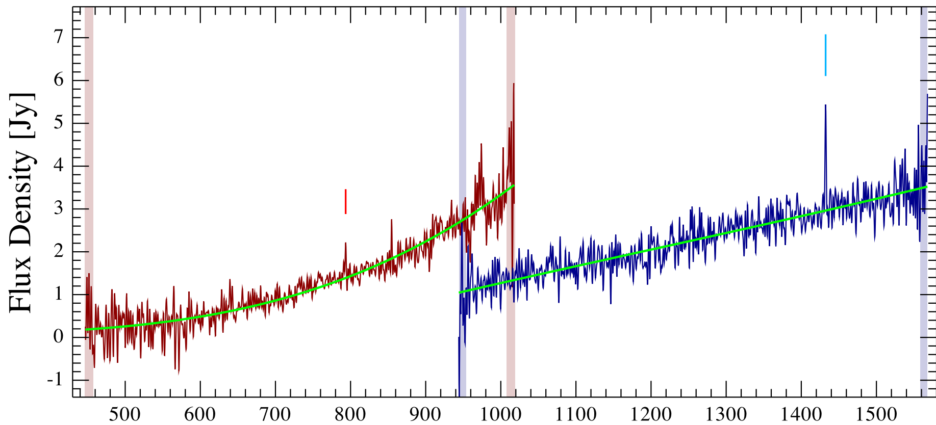
NGC6926 Observation ID 1342231050; (1/1)
