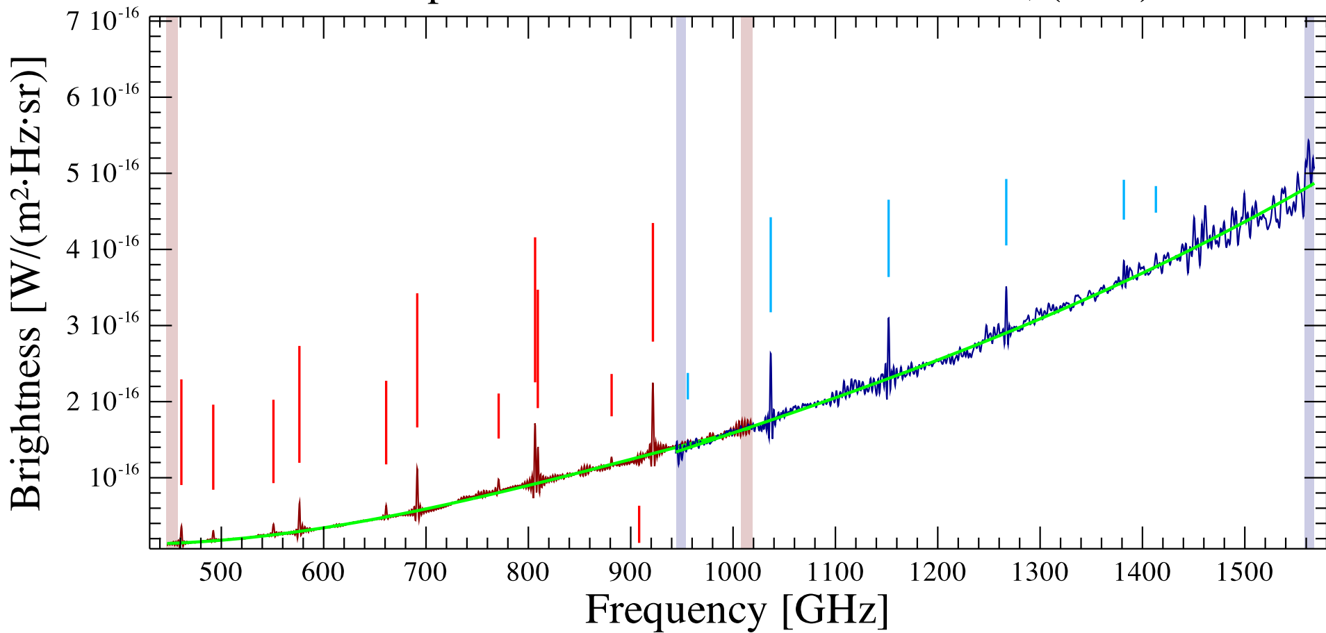
M 17 pos8 Observation ID 1342231045; (12/6)
