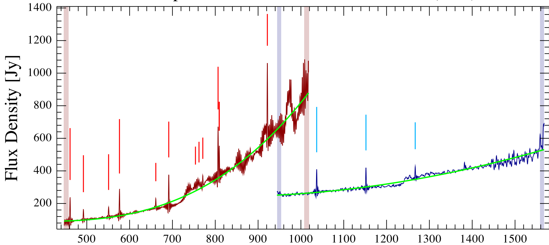
M 17 pos8 Observation ID 1342231045; (12/6)
