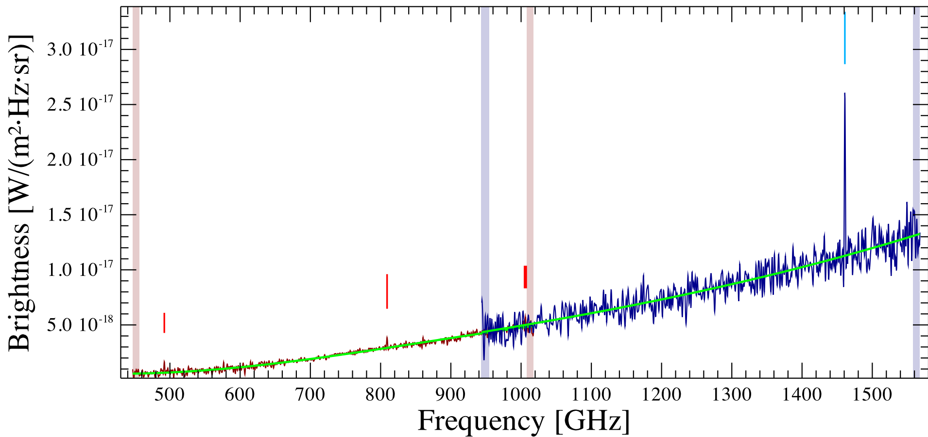
NGC 6567 Observation ID 1342231044; (3/1)
