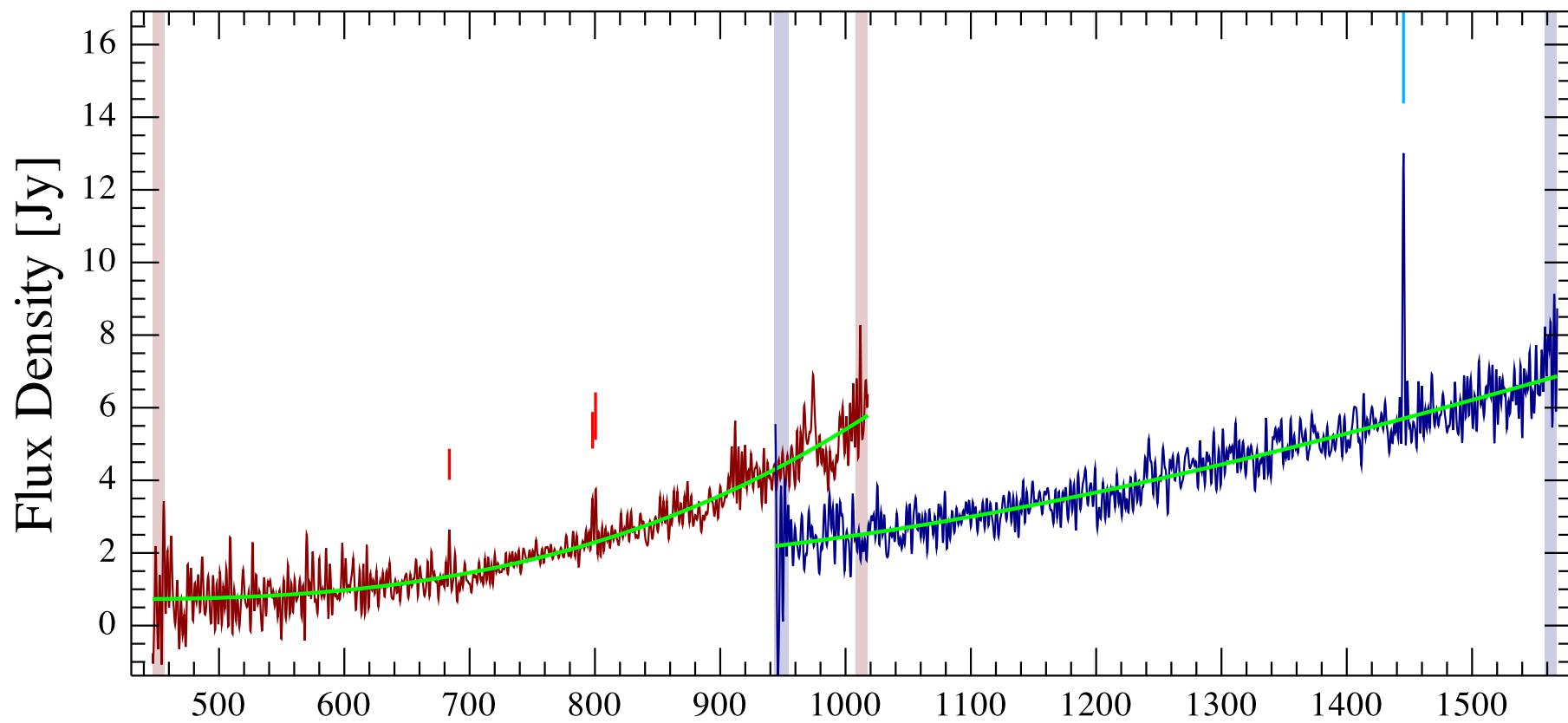
NGC6156 Observation ID 1342231041; (3/1)
