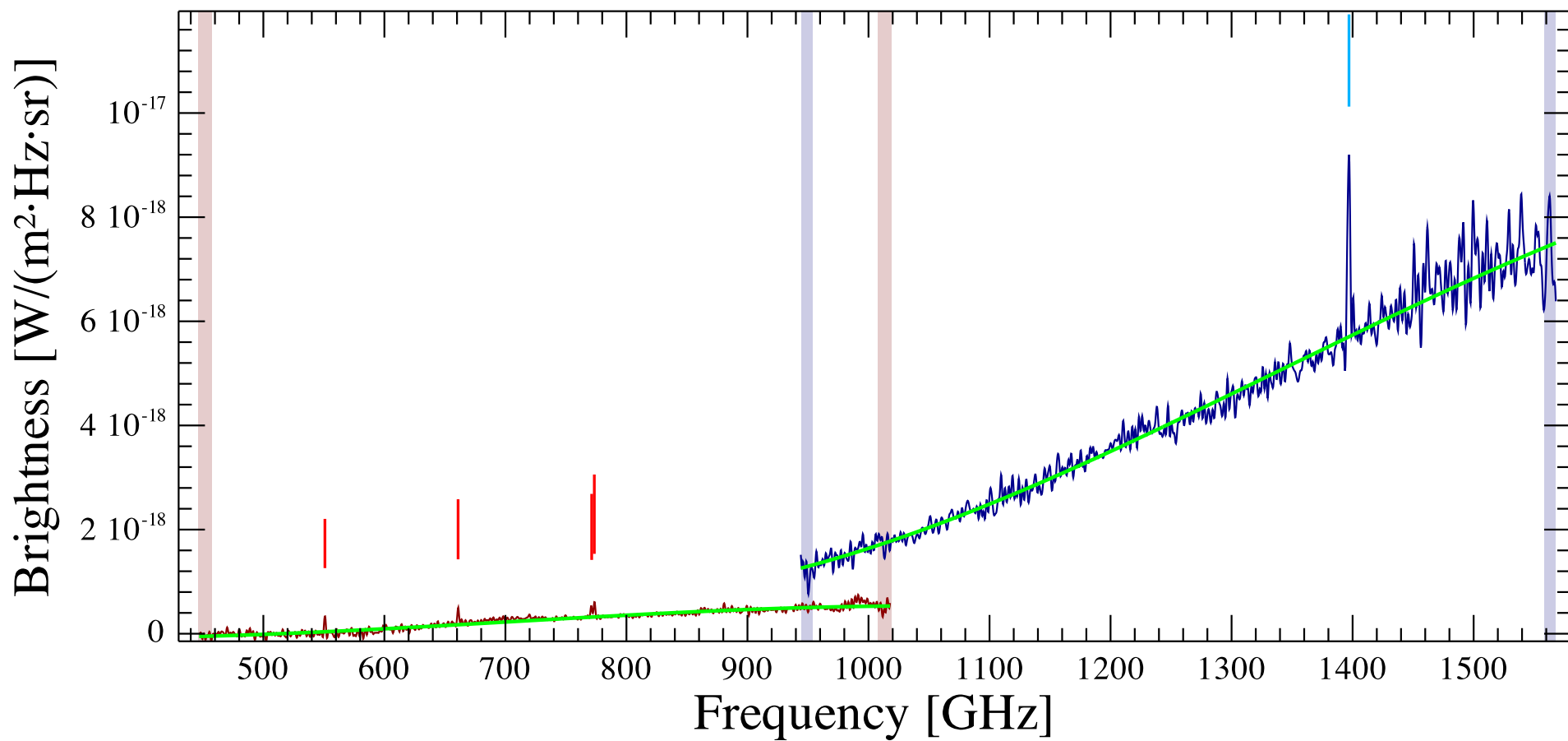
ESO069-IG006 Observation ID 1342231040; (4/1)
