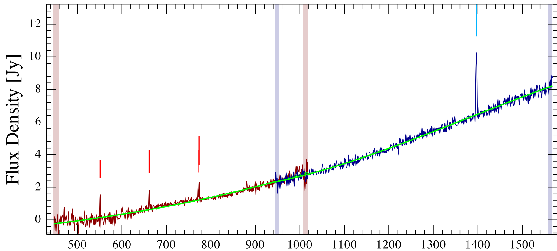
ESO069-IG006 Observation ID 1342231040; (4/1)
