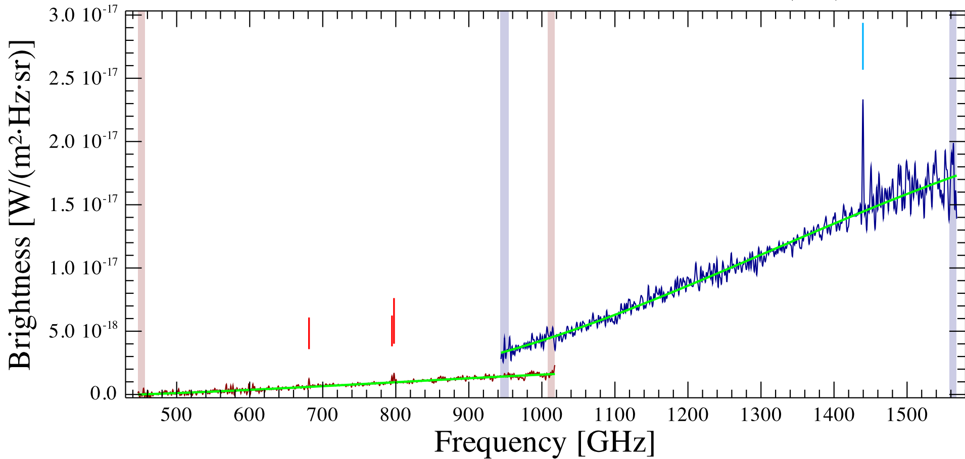
UGC03351 Observation ID 1342230415; (3/1)
