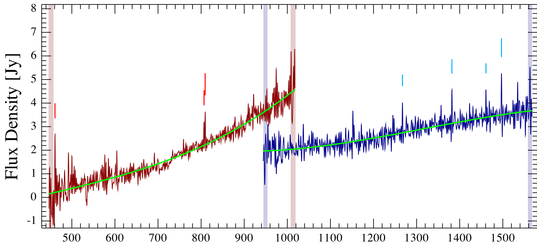
FU Orionis Observation ID 1342230412; (3/4)
