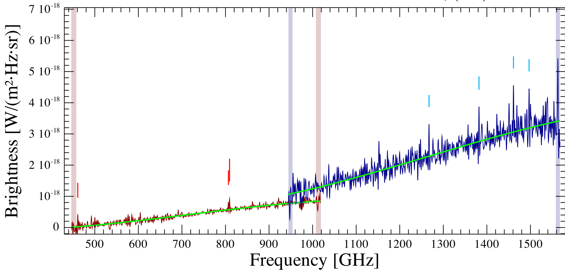
FU Orionis Observation ID 1342230412; (3/4)
