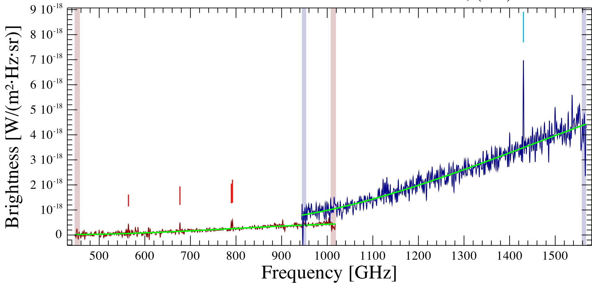
UGC03608 Observation ID 1342228744; (4/1)
