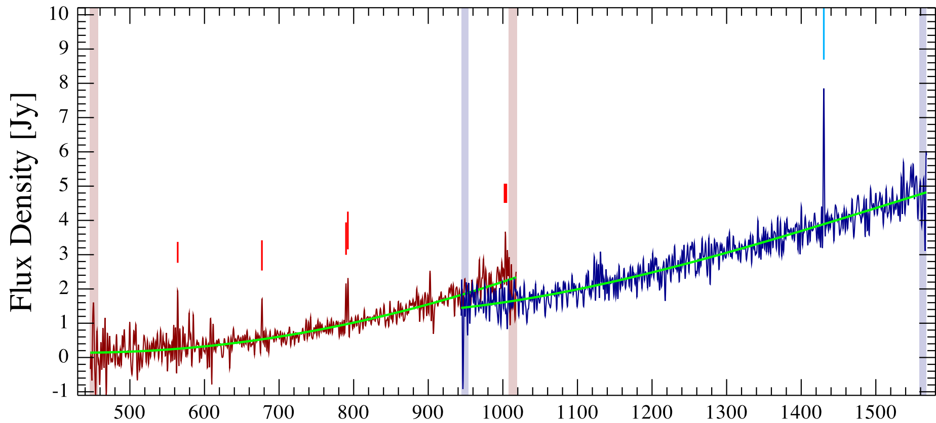
UGC03608 Observation ID 1342228744; (4/1)
