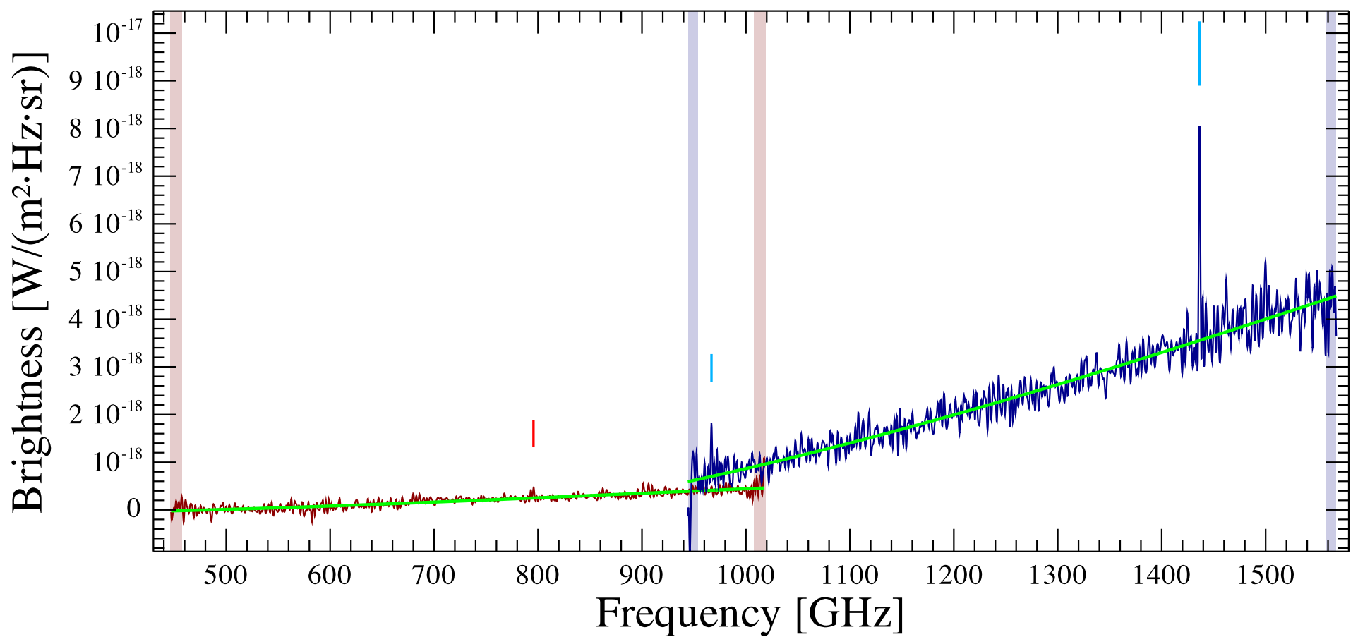
NGC2342b Observation ID 1342228730; (1/2)
