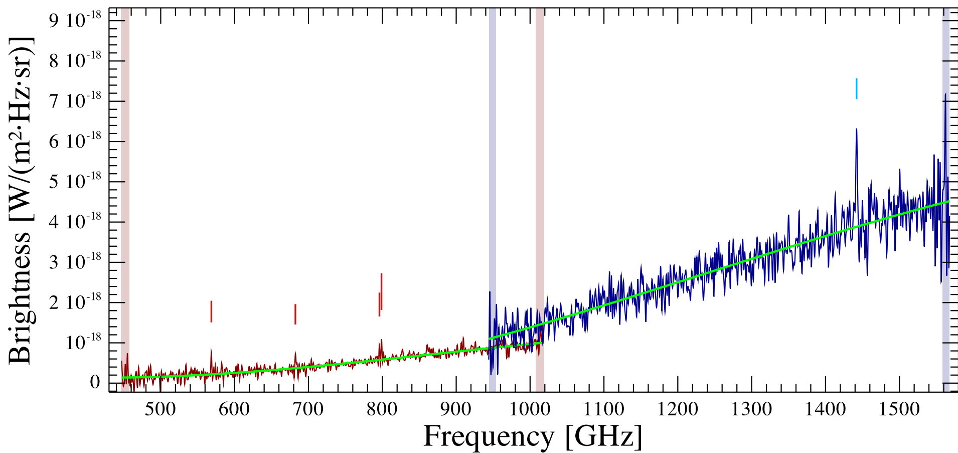
NGC1961 Observation ID 1342228708; (4/1)
