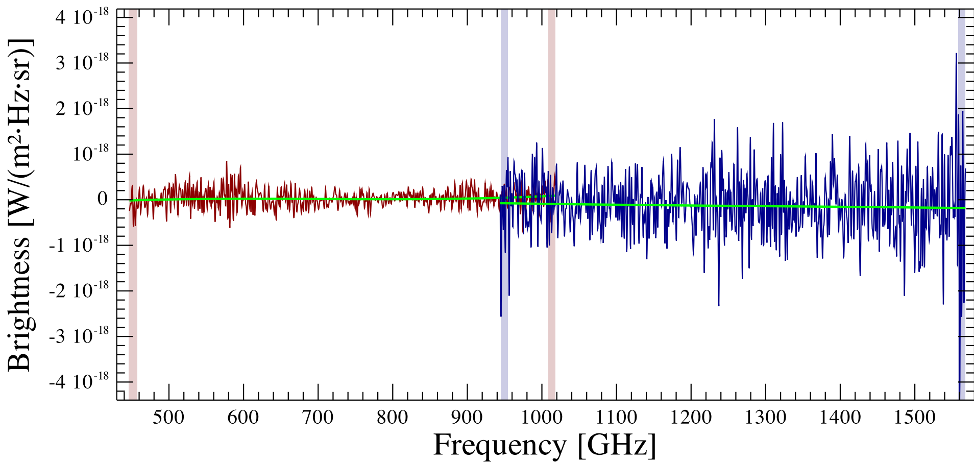
NGC 6543 OFF Observation ID 1342227788; (0/0)
