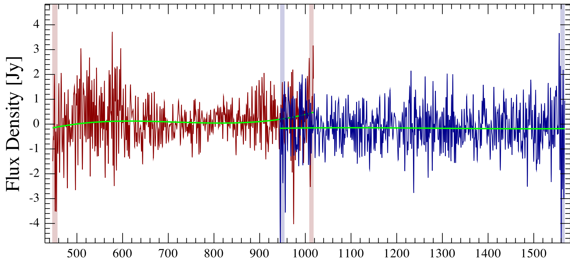
NGC 6543 OFF Observation ID 1342227788; (0/0)
