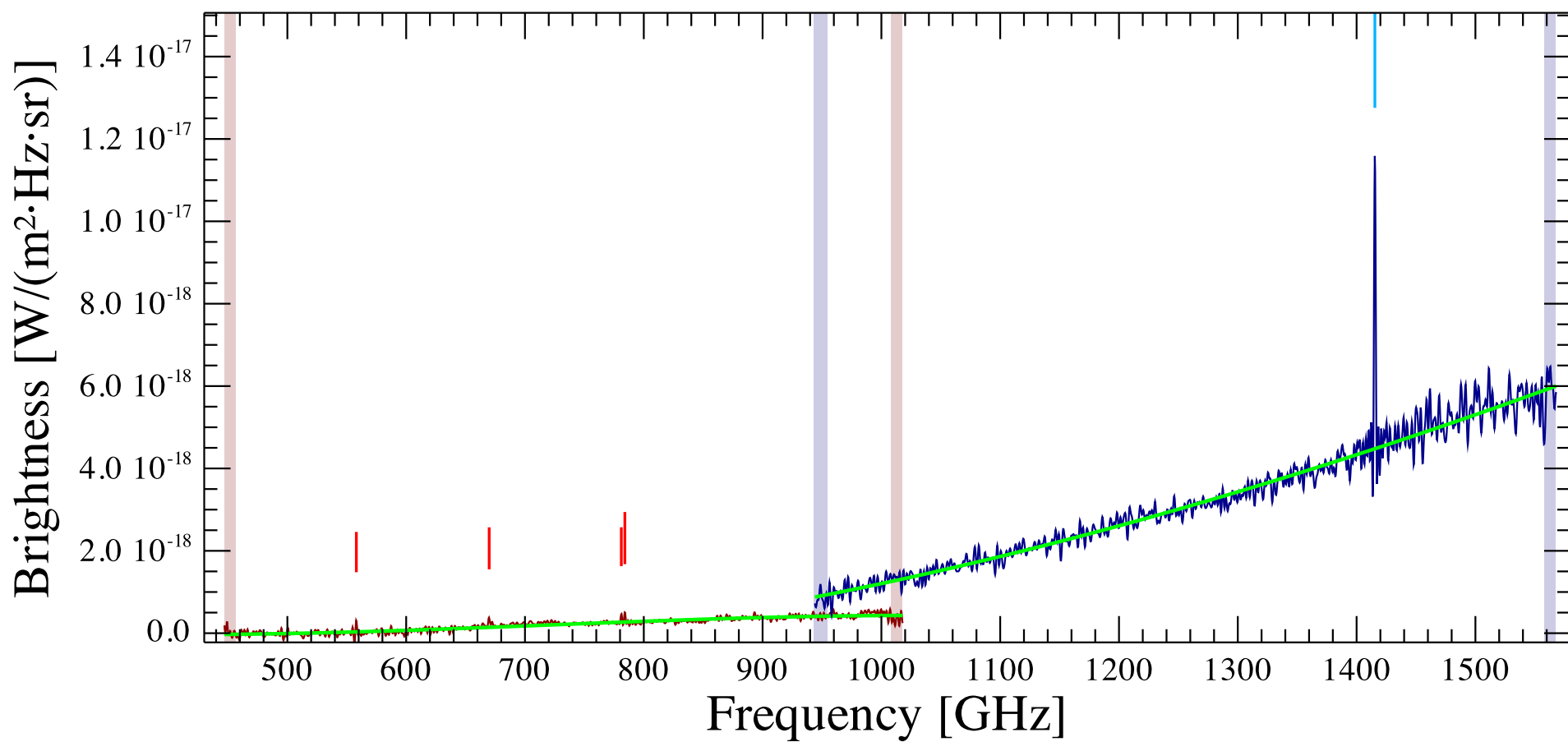
NGC0695 Observation ID 1342224767; (4/1)
